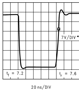
FIGURE 5. LM2437 Pulse Response
