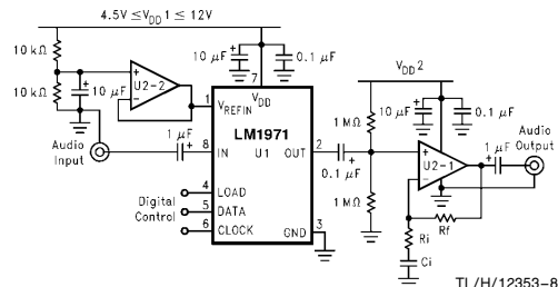
FIGURE 7. Active Reference with Active Gain Buffering
