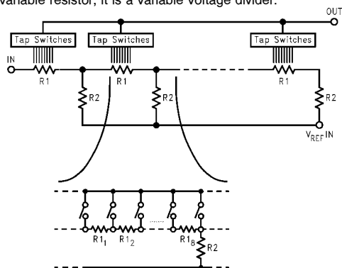
FIGURE 4. Resistor Ladder Architecture
