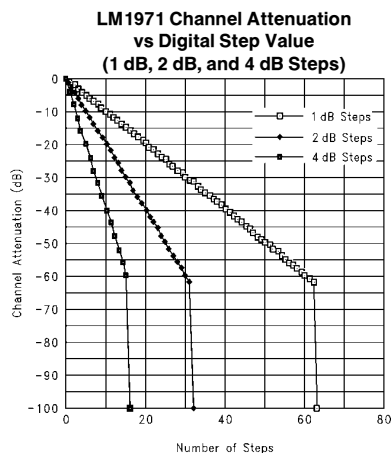
FIGURE 5. LM1971 Attenuation Step Scheme
