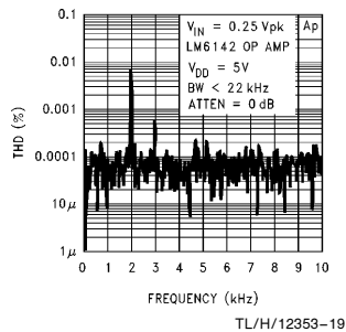
THD vs Freq by FFT
