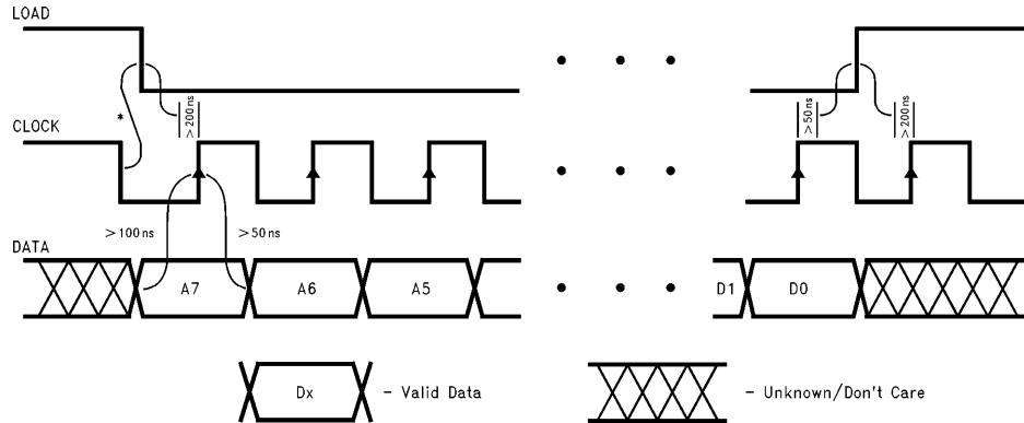
FIGURE 2. Timing Diagram
