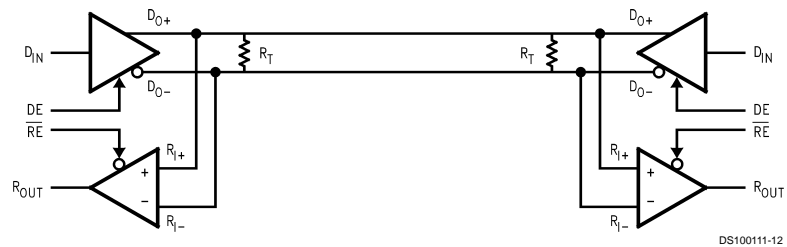
Bi-Directional Half-Duplex Point-to-Point Applications
