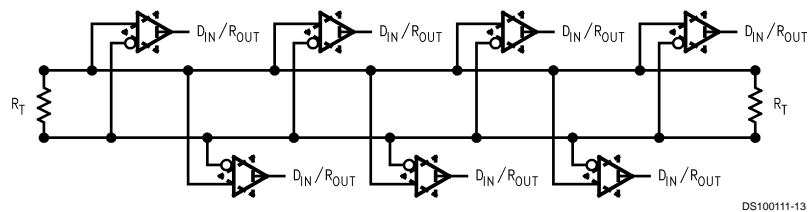
Multi-Point Bus Applications
