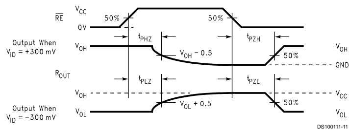
FIGURE 9. Receiver TRI-STATE Delay Waveforms
