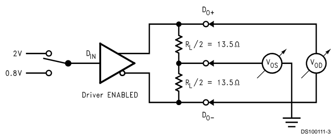
FIGURE 1. Differential Driver DC Test Circuit
