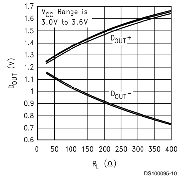
FIGURE 8. Typical DS90LV031A, D OUT (single ended) vs R L , T A = 25°C
