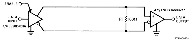
FIGURE 6. Point-to-Point Application
