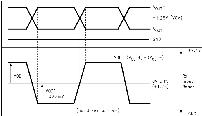
FIGURE 20. Single-Ended and Differential Waveforms
