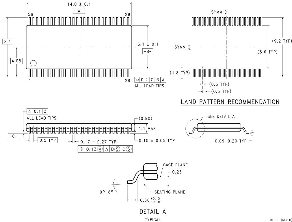
56-Lead Molded Thin Shrink Small Outline Package, JEDEC Order Number DS90C383, DS90CF384 NS Package Number MTD56
