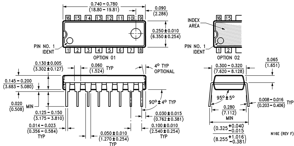
16-Lead Molded Dual-In-Line Package (N) DS26F31CN NS Package Number N16E
