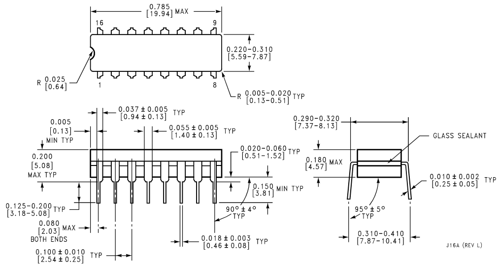
16-Lead Ceramic Dual-In-Line Package (J) DS26F31CJ or DS26F31MJ/883 NS Package Number J16A
