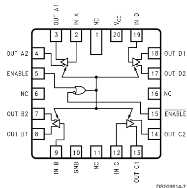
FIGURE 1. Logic Symbol
