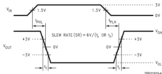
FIGURE 2. Driver Propagation Delay and Slew Rate Timing
