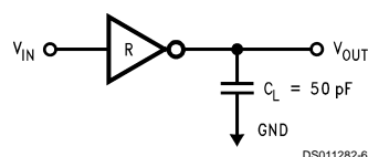
FIGURE 3. Receiver Load Circuit
