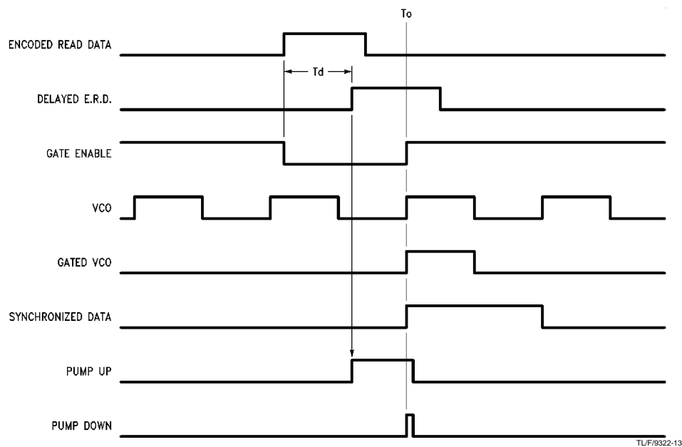
FIGURE 8. Capture of Early-Shifted ENCODED READ DATA Pulse
