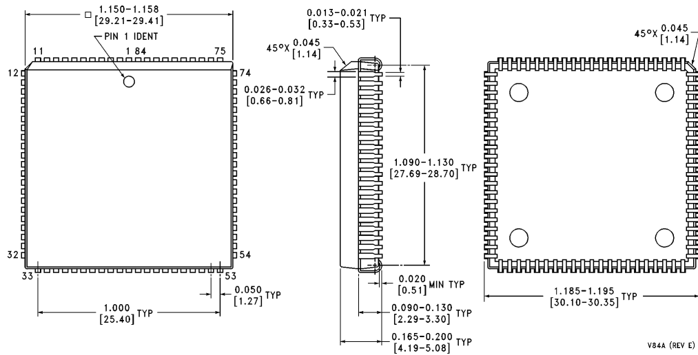
Plastic Chip Carrier (V) Order Number DP83955AV NS Package Number V84A
