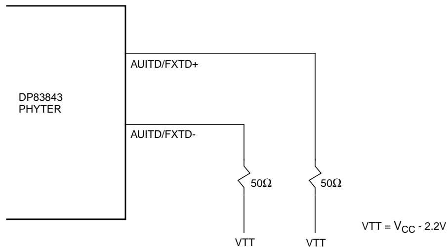
Figure 26. 100BASE-FX Test Load
