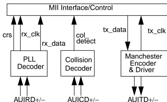
Figure 13. AUI Block Diagram
