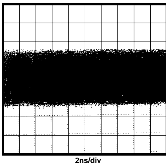
Figure 9. MLT-3 Signal Measured at All after 100 meters of CAT-5 cable
