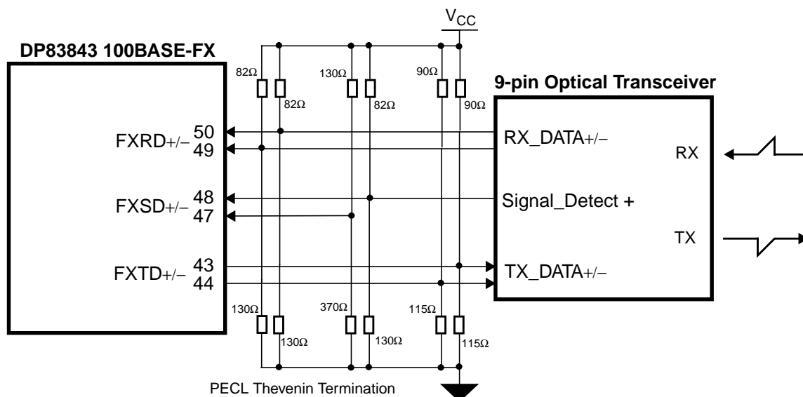
Figure 12. Typical DP83843 to Optical Transceiver Interfaces
