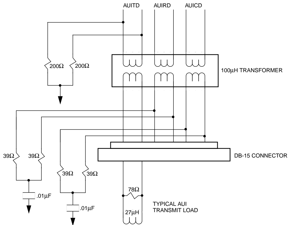
Figure 25. AUI Test Load
