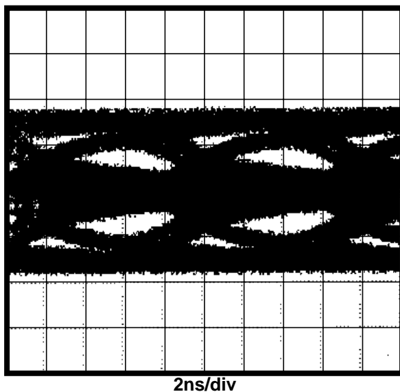
Figure 8. MLT-3 Signal Measured at All after 50 meters of CAT-5 cable
