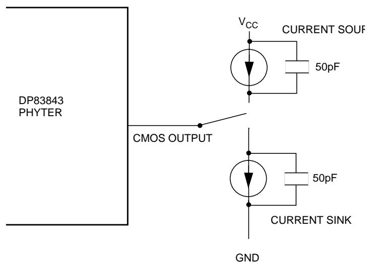
Figure 27. CMOS Output Test Load
