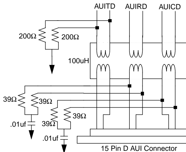
Figure 14. AUI Typical Setup
