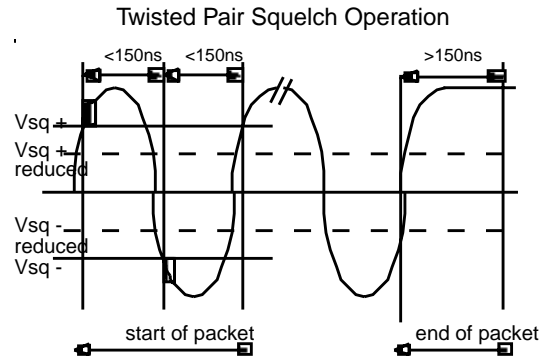
Figure 10. 10BASE-T Twisted Pair Smart Squelch Operation
