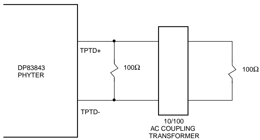
Figure 28. 10/100 Twisted Pair Load (zero meters)
