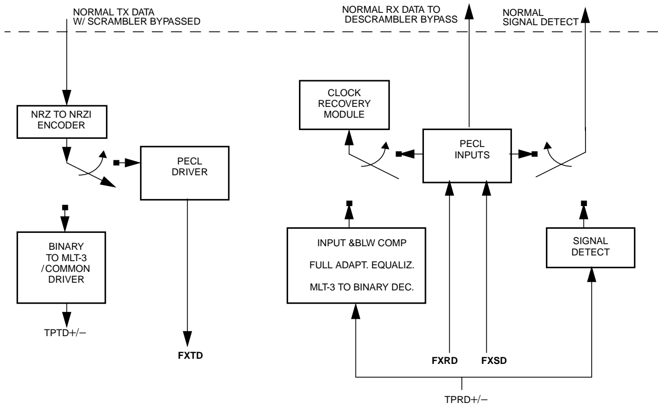
Figure 11. 100Base-FX Block Diagram
