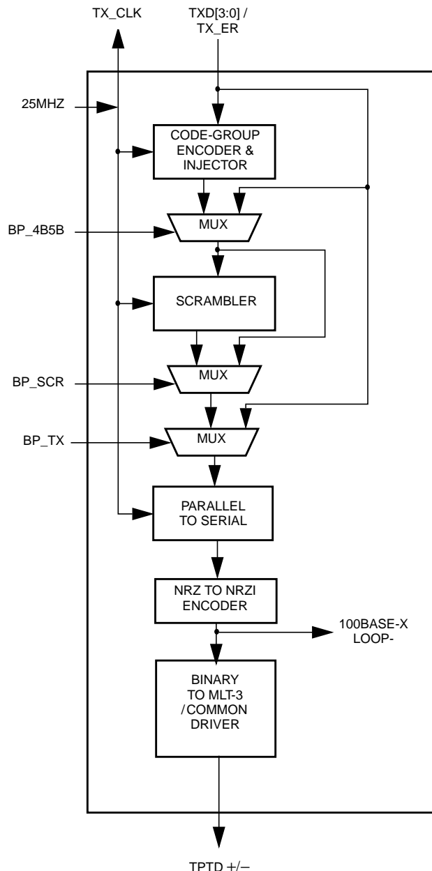
Figure 3. 100BASE-TX Transmit Block Diagram
