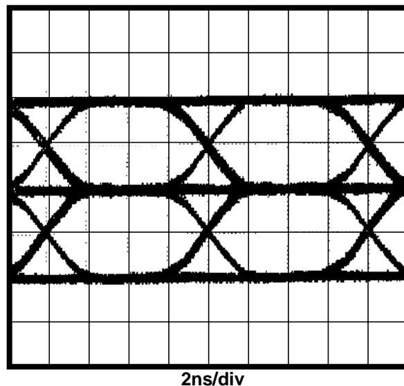
Figure 7. MLT-3 Signal Measured at All after 0 meters of CAT-5 cable
