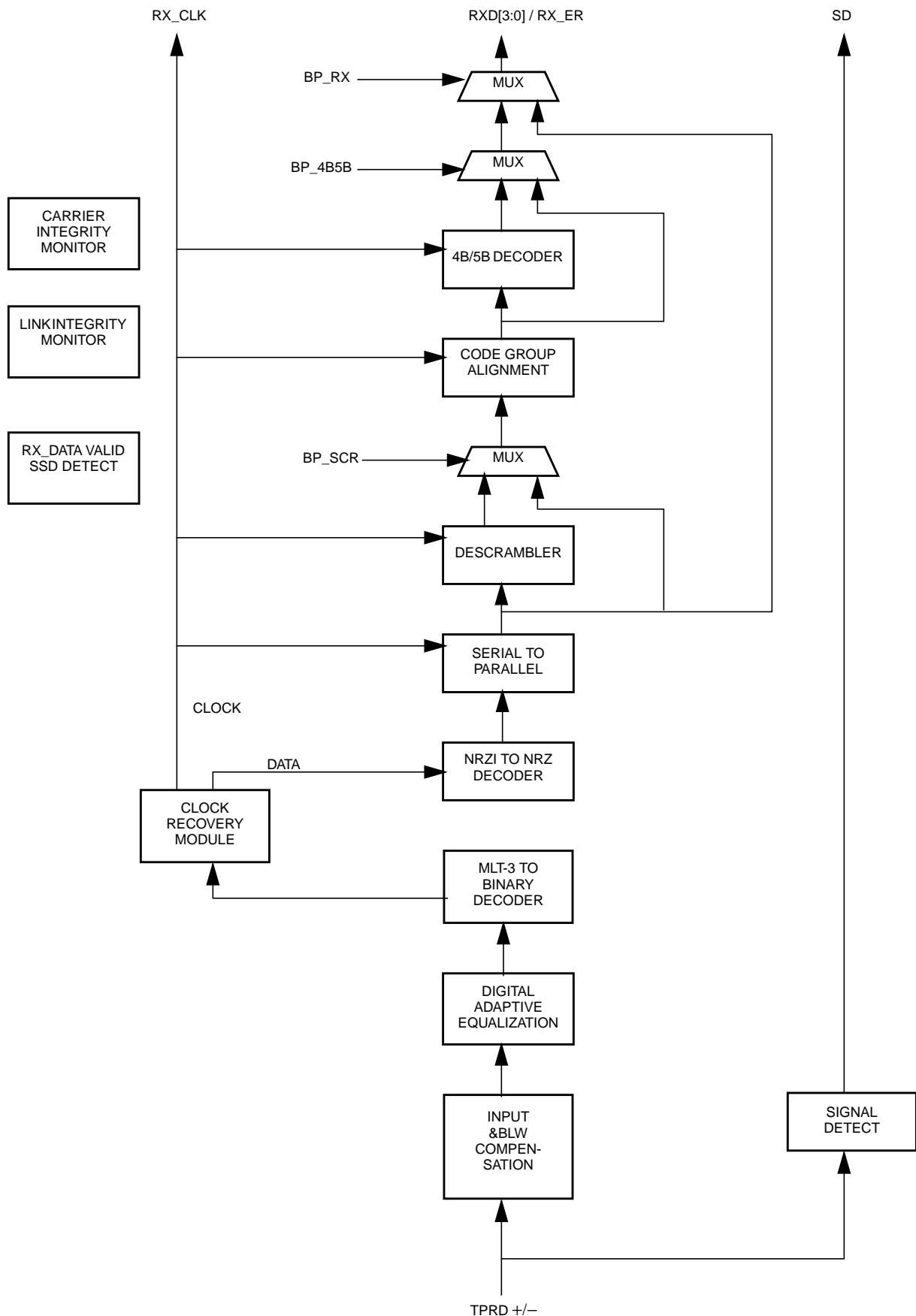
Figure 5. Receive Block Diagram
