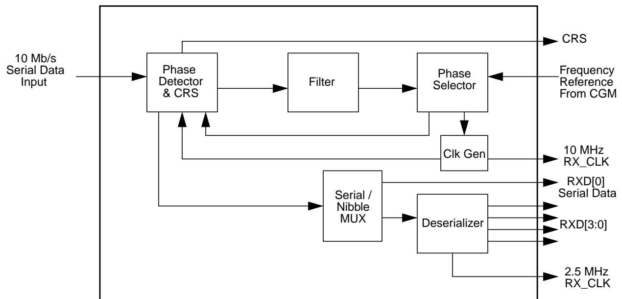
Figure 19. 10M Manchester Clock Recovery Module block diagram
