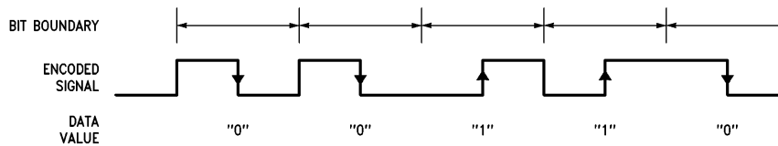
FIGURE 1-1. Biphas Encoding
