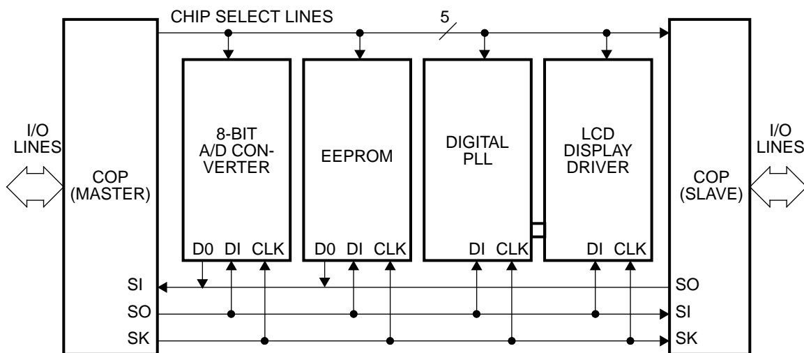
Figure 14. MICROWIRE/PLUS Application
