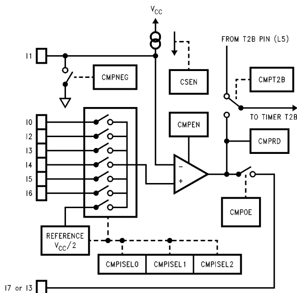
FIGURE 12. COP87L88EK Analog Function Block
