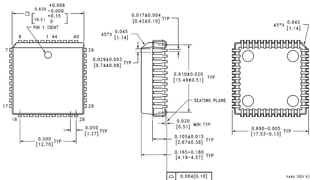
Plastic Leaded Chip Carrier (V) Order Number COP87L88EKV-XE NS Package Number V44A
