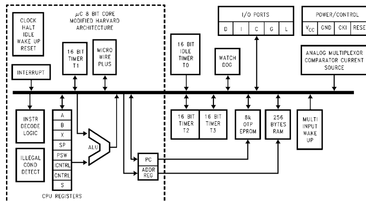
FIGURE 1. Block Diagram
