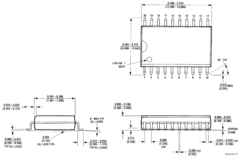
20-Lead Surface Mount Package (M) Order Number COP87L42CJM (-1B, -1N, -2B, -2N, -3B, -3N) NS Package Number M20B
