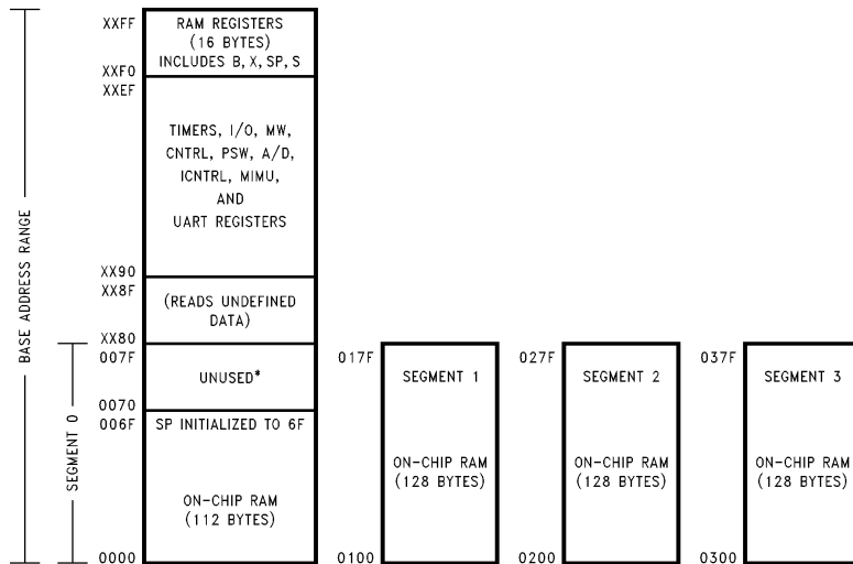
FIGURE 5. RAM Organization
