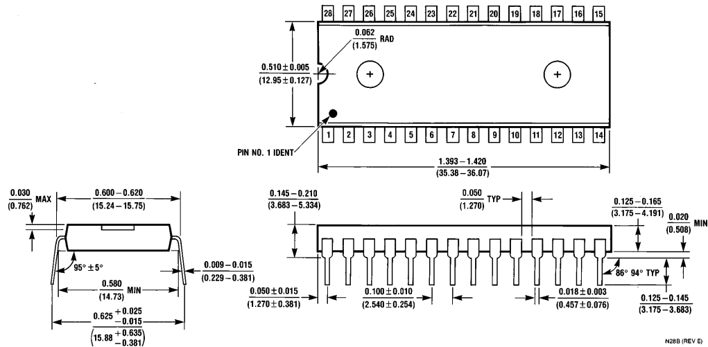
Molded Dual-In-Line Package (N) Order Number COP684FH-XXX/N, COP884FH-XXX/N or COP984FH-XXX/N NS Package Number N28A
