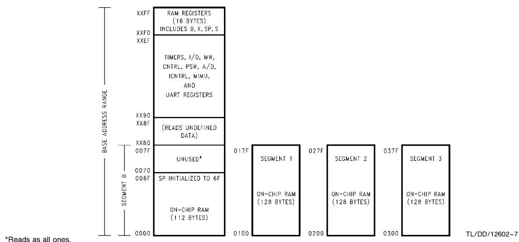
FIGURE 5. RAM Organization
