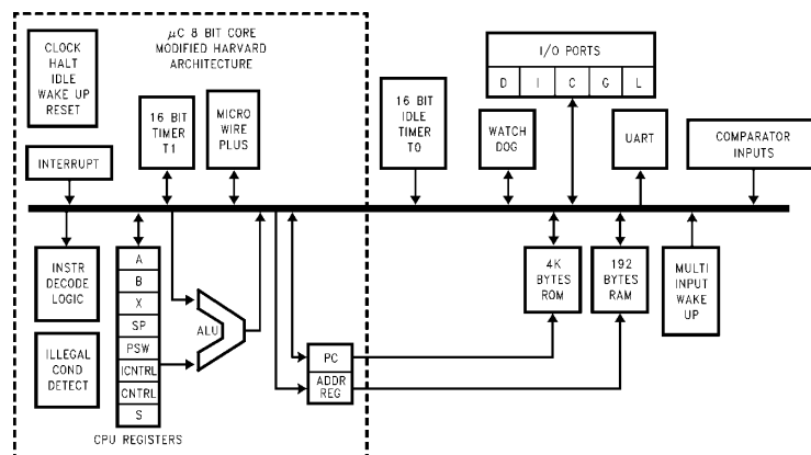
FIGURE 1. Block Diagram
