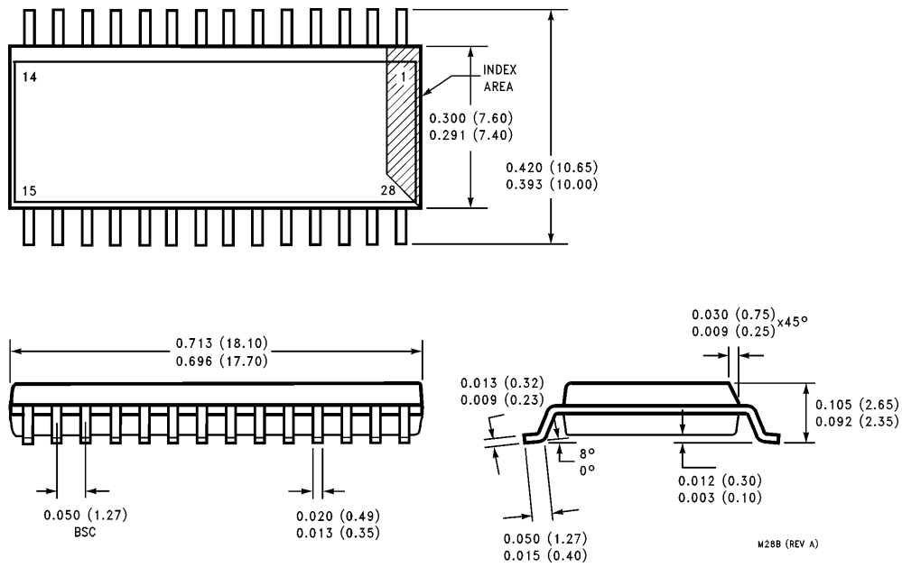
28-Lead Small Outline Wide Body Package (M) Order Number COP884CS-XXX/WM, COP984CS-XXX/WM or COP984CSH-XXX/WM NS Package Number M28B
