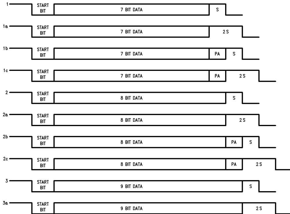
FIGURE 13. Framing Formats
