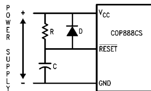
FIGURE 6. Recommended Reset Circuit
