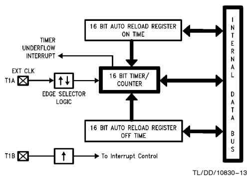
FIGURE 9. Timer in External Event Counter Mode
