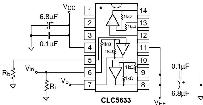
Figure 7: Dual Supply, A_v = -1V/V Configuration
