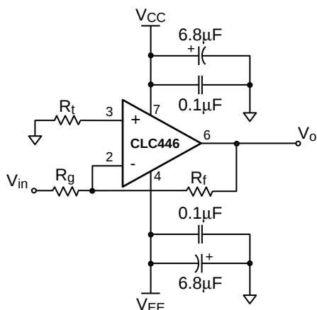
Figure 2: Inverting Gain
