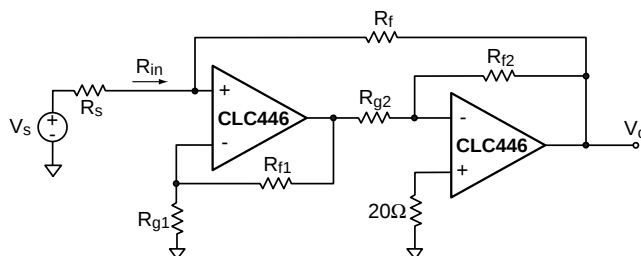
Figure 10: Composite Amplifier
