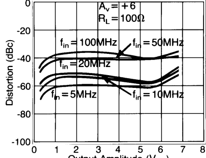
2nd Harmonic Distortion, C_L = 25pF
