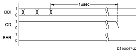
FIGURE 10. Input Data Removed
