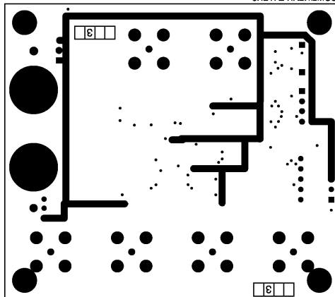
COMLINEAR LAYER1 SILK
