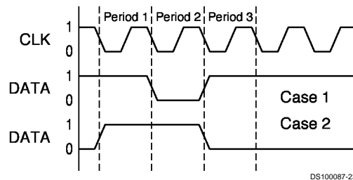
FIGURE 11. Harmonic Lock Detector Operation
