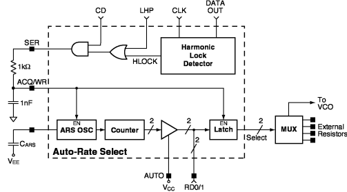
FIGURE 7. Auto-Rate Select
