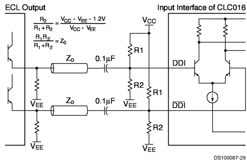
FIGURE 17. AC Coupled Termination
