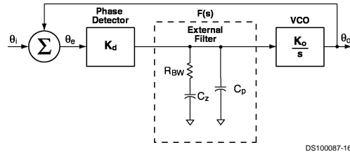
FIGURE 4. PLL Loop
