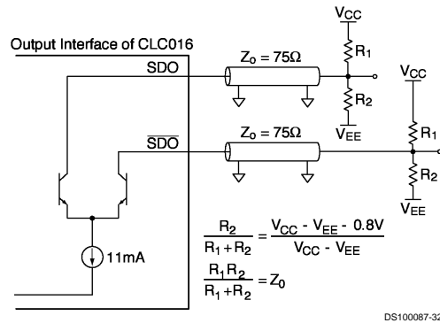
FIGURE 20. Load Terminated Output Interface
