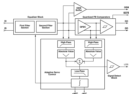
FIGURE 2. CLC012 Block Diagram
