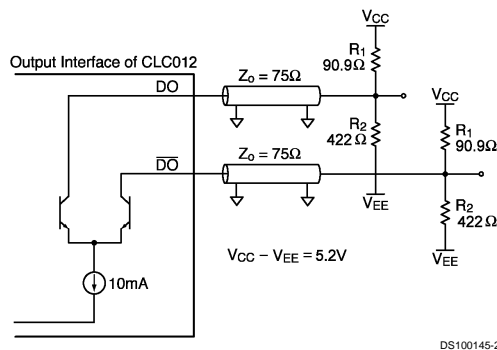
FIGURE 7. Alternative Load Terminated Output Interface
