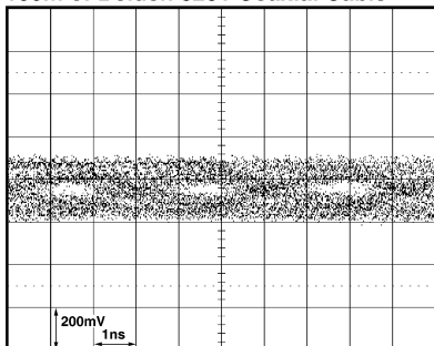
Before Equalization: 155Mbps 100m of Belden 8281 Coaxial Cable
