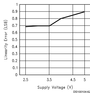
Integral Linearity Error vs Supply Voltage
