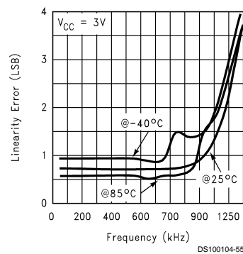
Linearity Error vs Clock Frequency
