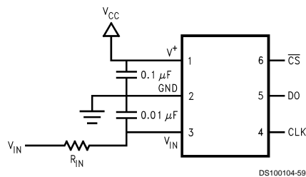
Recommended Power Supply Bypassing
