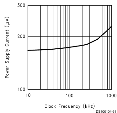
Power Supply Current vs Clock Frequency
