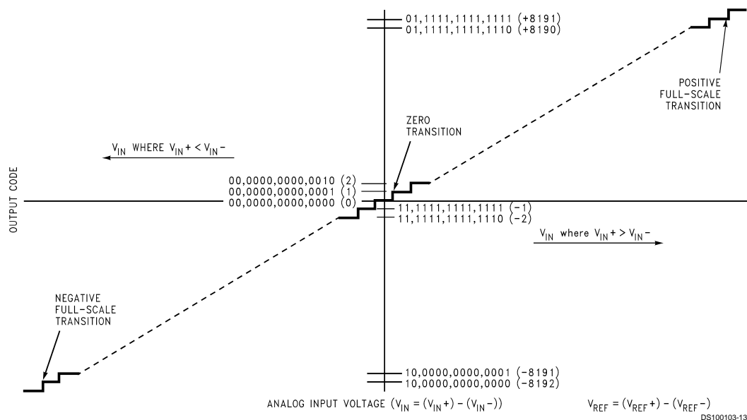
FIGURE 1. Transfer Characteristics
