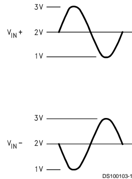
FIGURE 4. Expected Input Signal Range.
