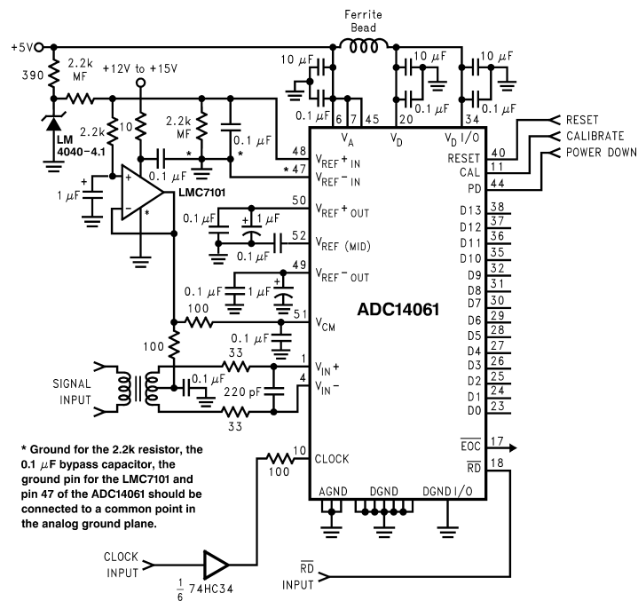
FIGURE 8. Driving the signal inputs with a transformer.
