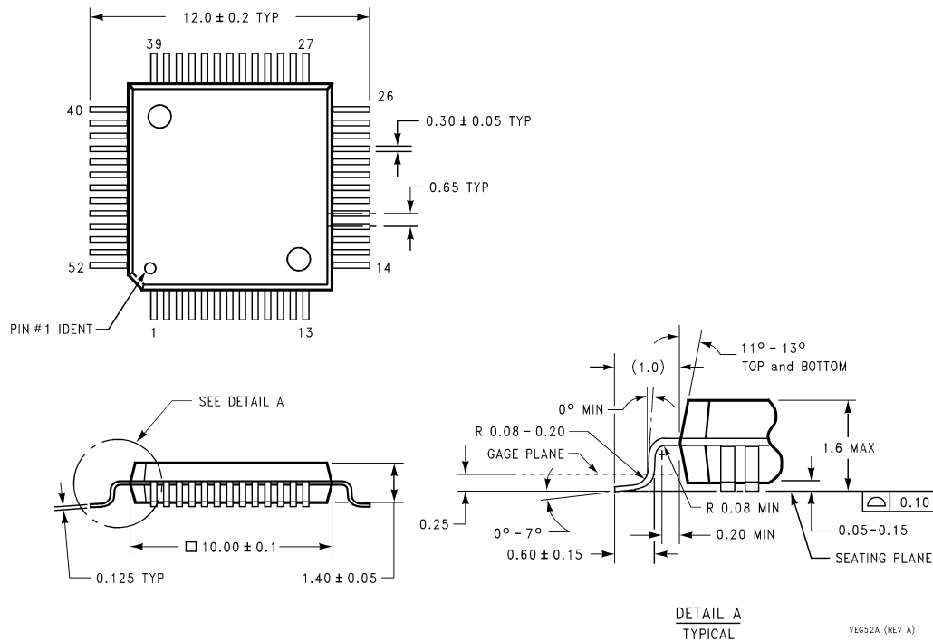
52-Lead Thin Quad Flat Pack Ordering Information Package ADC14061CCVT NS Package Number VEG52A
