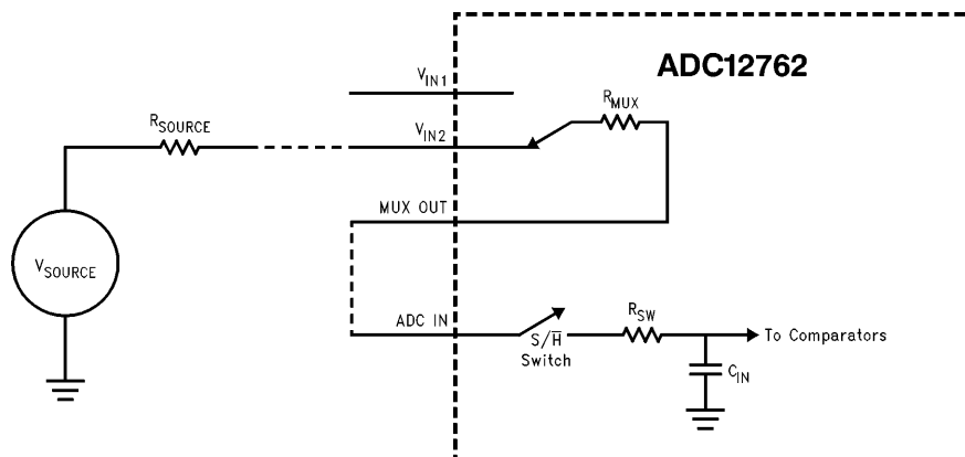
FIGURE 7. Simplified ADC12762 Input Stage
