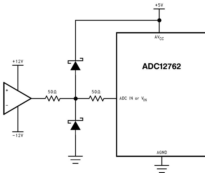
FIGURE 9. Input Protection
