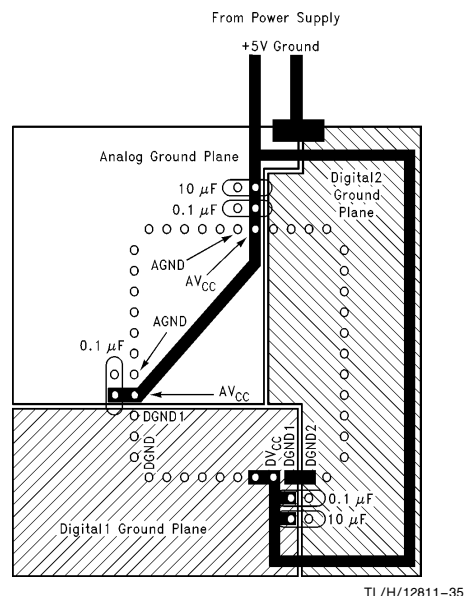
FIGURE 12. PC Board Layout
