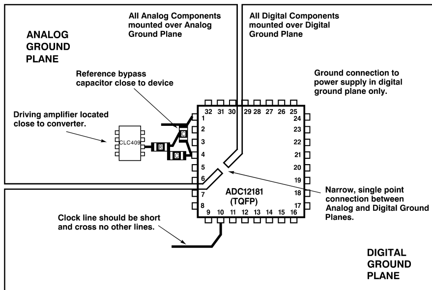
FIGURE 6. Layout example
