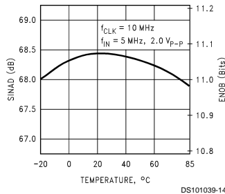
SINAD vs Temperature
