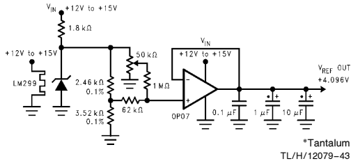
FIGURE 14. Low Drift Extremely Stable Reference Circuit
