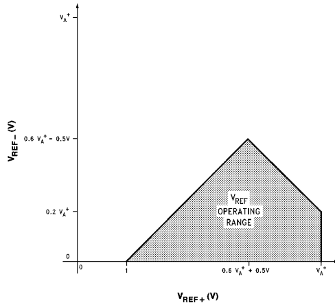
FIGURE 15. V_{REF} Operating Range
