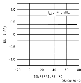
DNL vs Temperature
