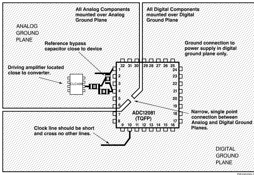
FIGURE 6. Layout example
