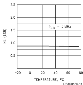
INL vs Temperature
