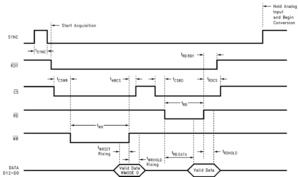
FIGURE 7d. Sync-In Write (WMODE = 0, BW = 1), Read and Convert Cycles
