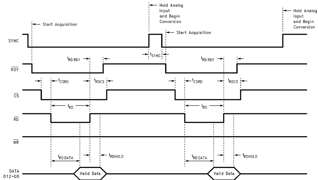
FIGURE 7f. Sync-In Read and Convert Cycles
