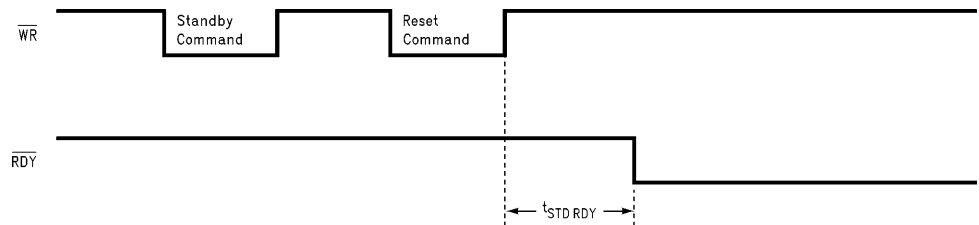
FIGURE 7j. Standby and Reset Timing (13-Bit Data Bus Width)
