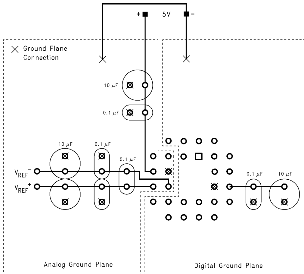
FIGURE 10. Top View of Printed Circuit Board for a 28-Pin PLCC ADC12041
