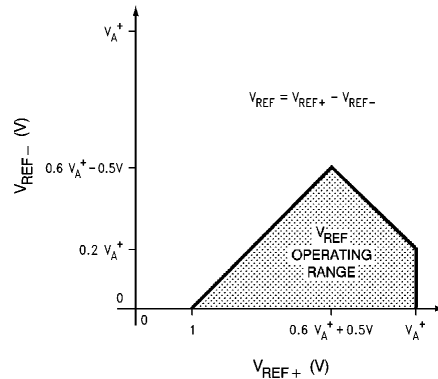
FIGURE 9. V_{REF} Operating Range
