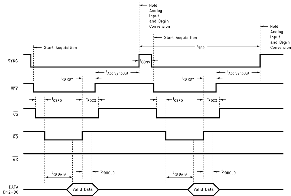
FIGURE 7e. Sync-Out Read and Convert Cycles
