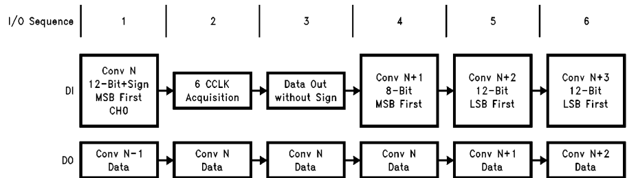
FIGURE 6. Changing the ADC's Conversion Configuration
