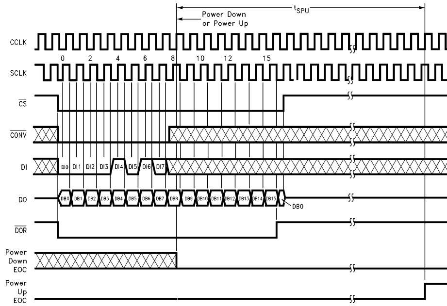
ADC12038 Software Power Up/Down Using \overline{\text{CS}} with 16-Bit Digital Output Format
