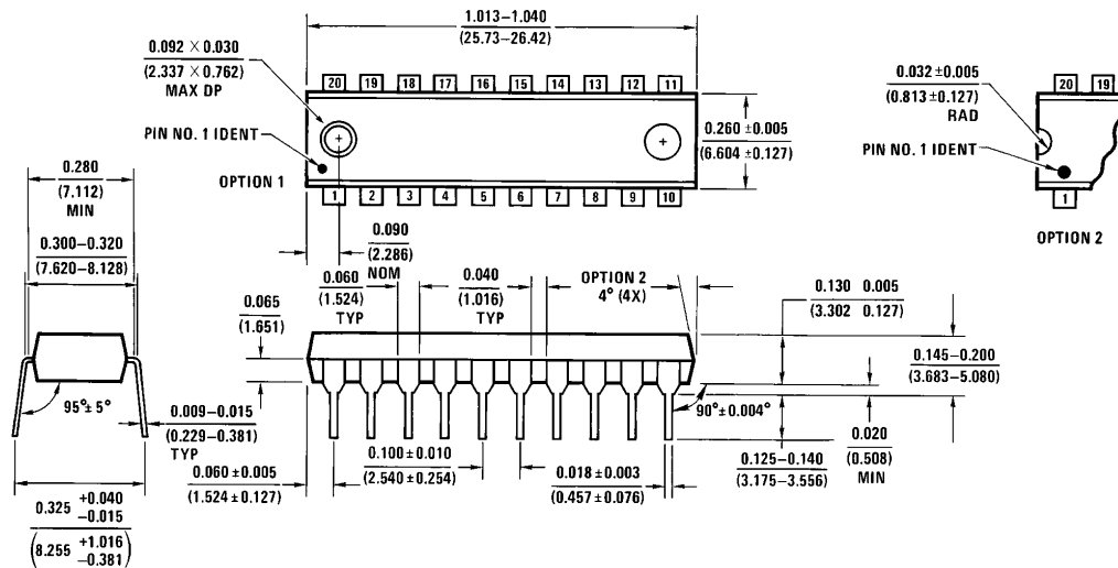
Order Number ADC12032CIN or ADC12H032CIN NS Package Number N20A
