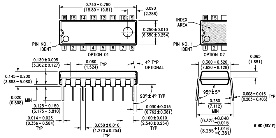
Order Number ADC12030CIN or ADC12H030CIN NS Package Number N16E
