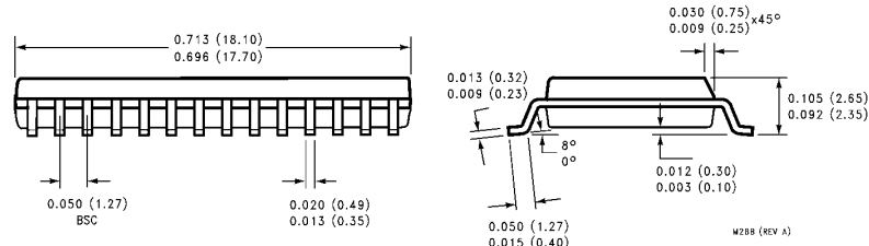
Order Number ADC10664CIWM NS Package Number M28B
