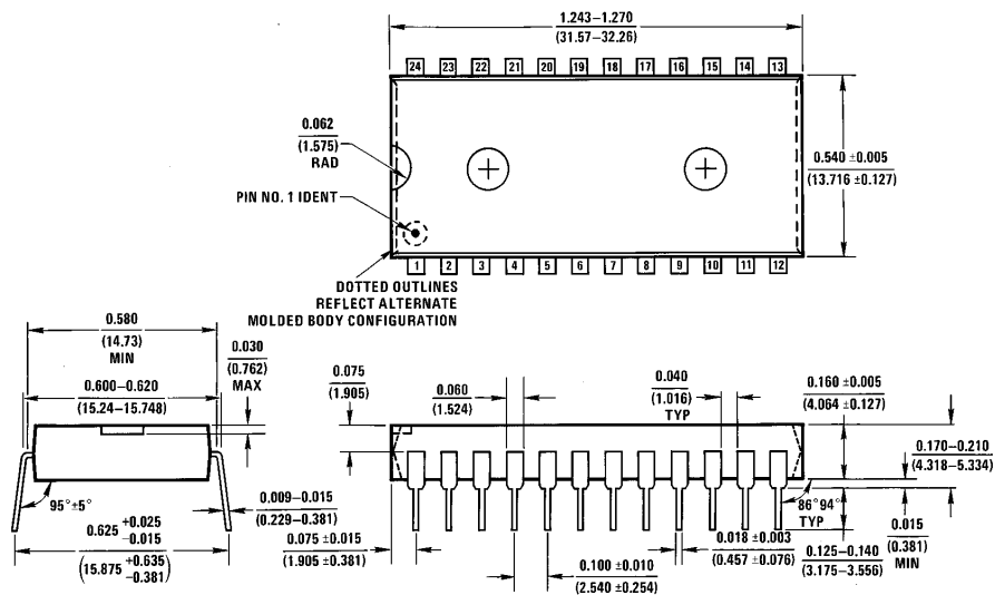
Order Number ADC10662CIN NS Package Number N24A
