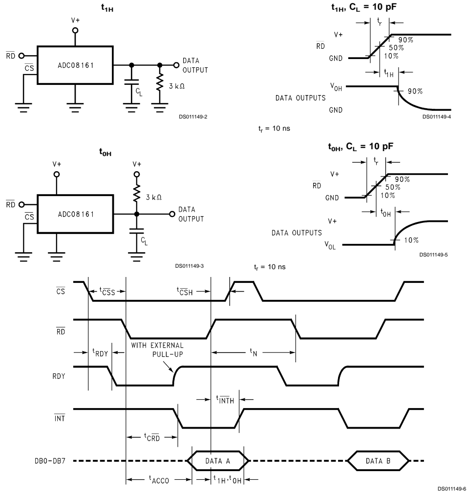
FIGURE 1. RD Mode (Mode Pin is Low)
