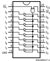
Pin Assignment DIP and Cerpac
