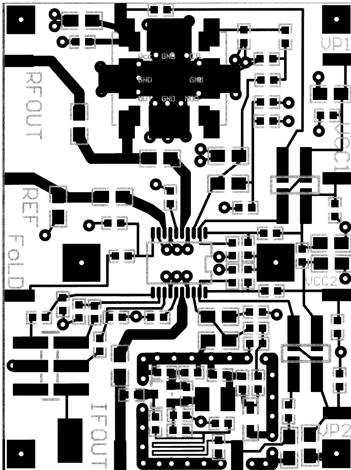
Figure 3 : LMX2332L Evaluation Board Layout
