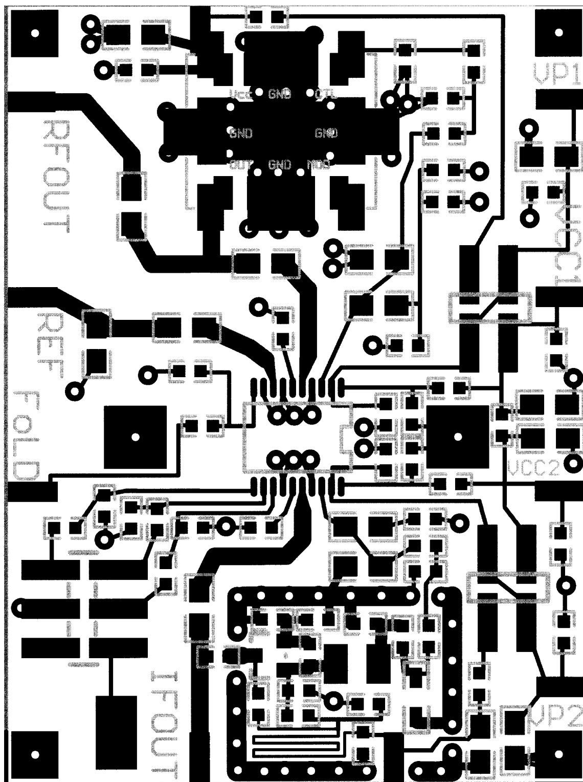
Figure 3 : LMX2332A Evaluation Board Layout
