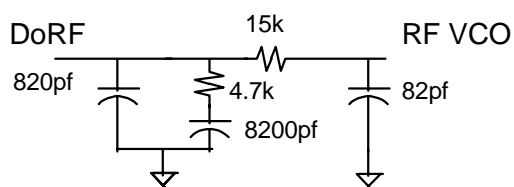
RF LOOP FILTER
