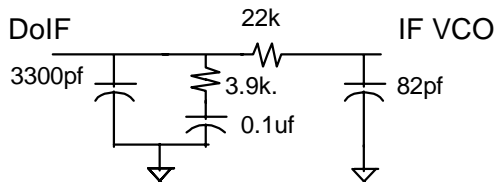
IF LOOP FILTER
