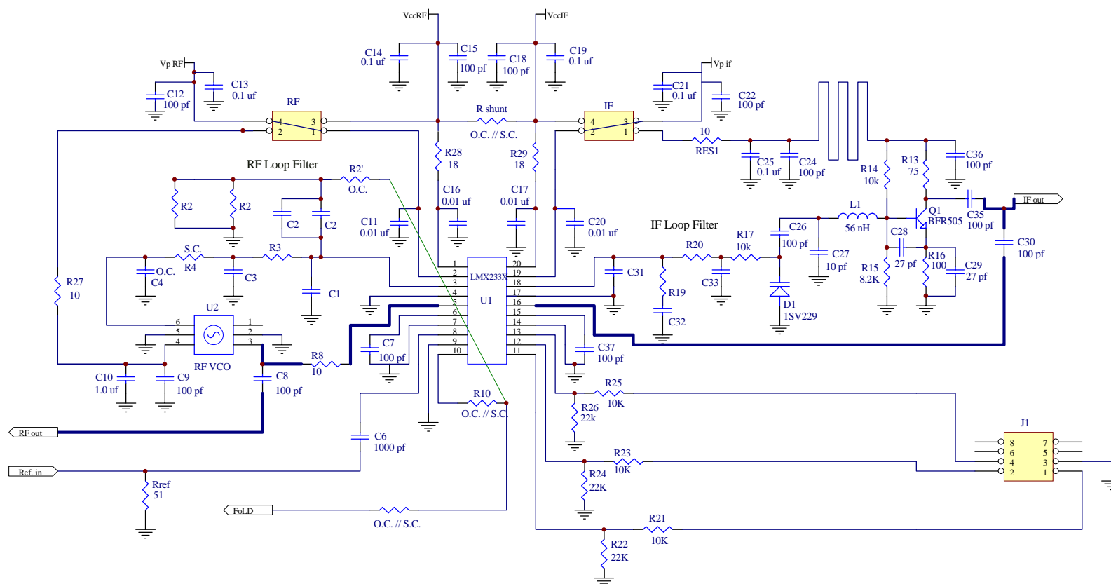
Dual PLL (20 Pin) Evaluation Board (3 Volt Operation)
