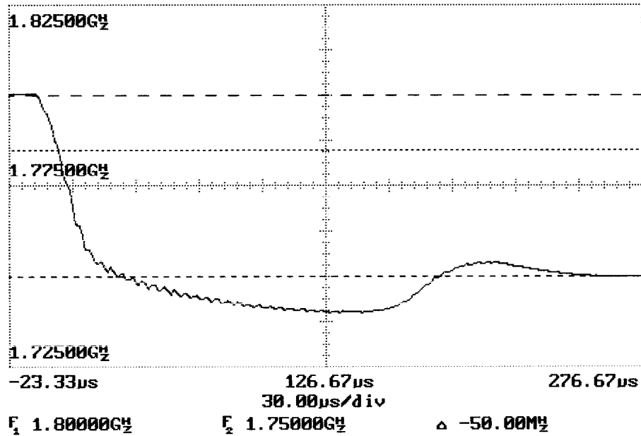
Negative Frequency Switching Waveform
