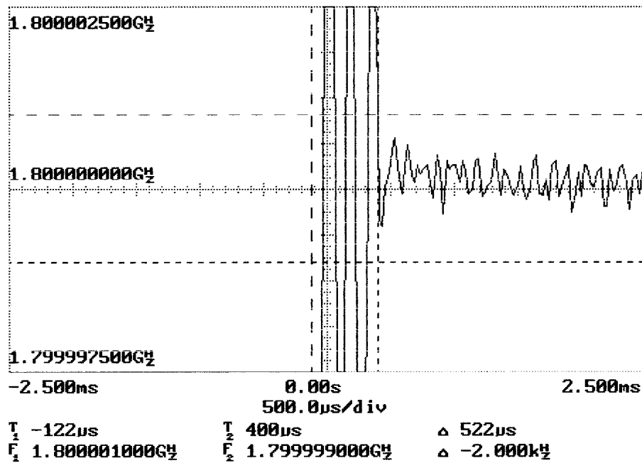
PositiveLock Time to within 1 kHz
