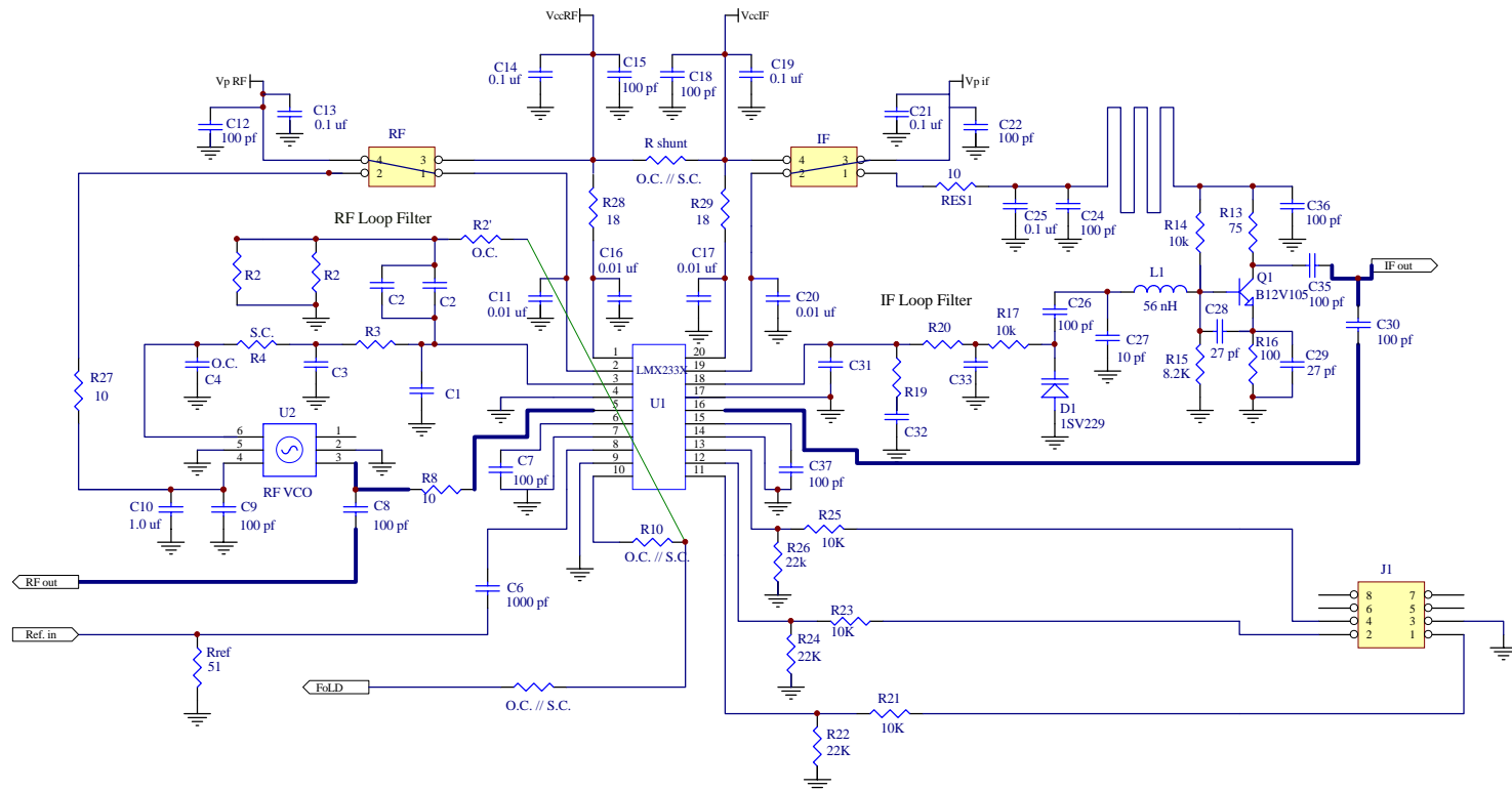
Dual PLL (20 Pin) Evaluation Board (3 Volt Operation)
