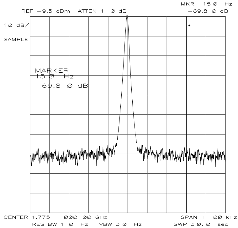
“Close in” Phase Noise
