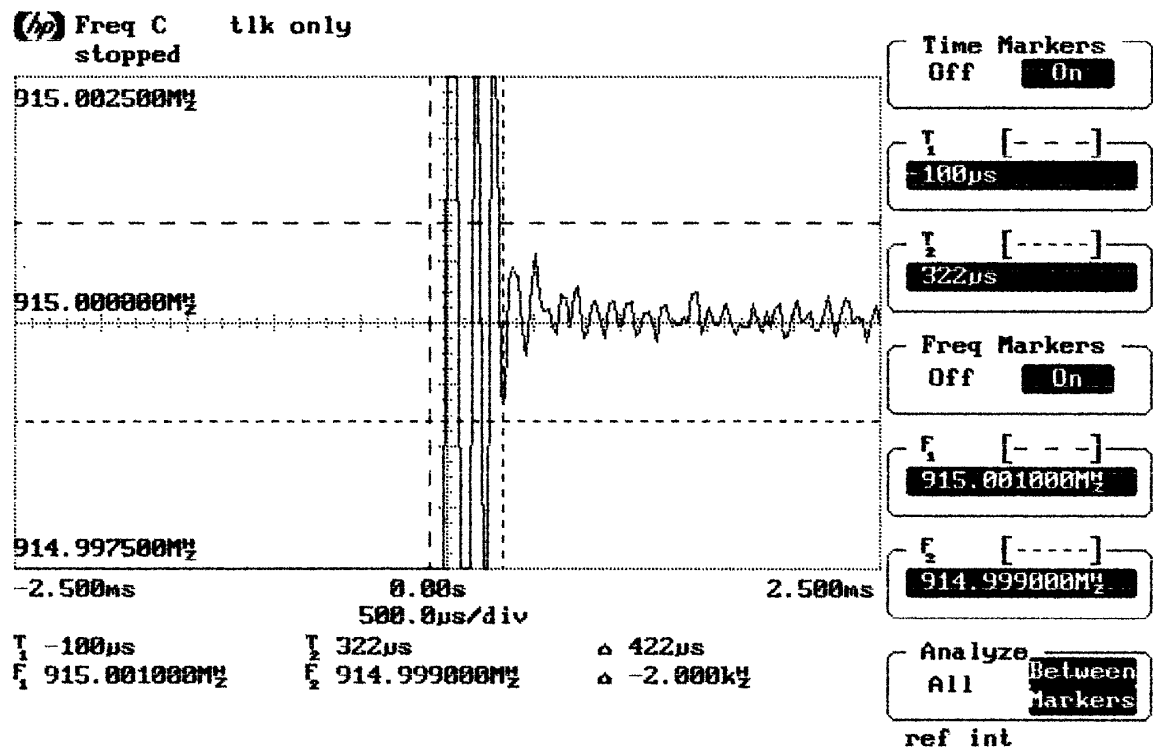
Positive Lock Time to within 1 kHz Range
