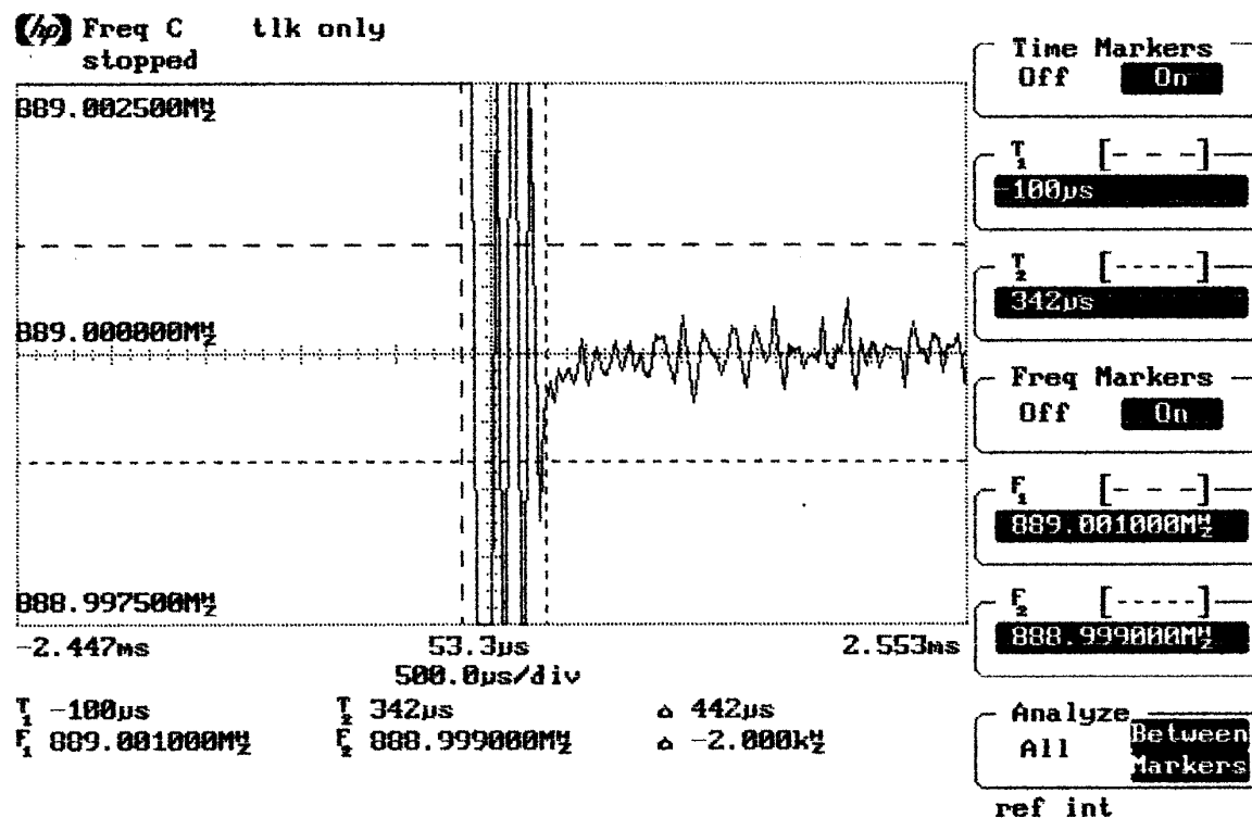
Negative Lock Time to within 1kHz Range
