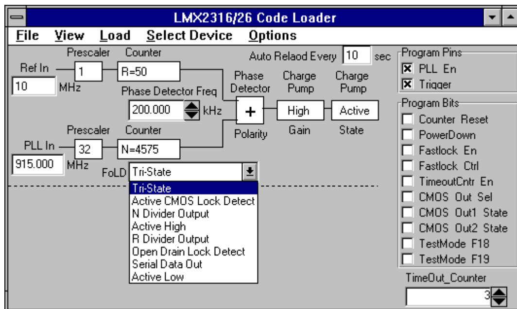
FIGURE D-1: "CODE LOADER" MAIN MENU FOR LMX2316
