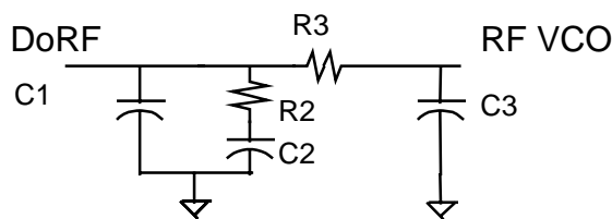
LOOP FILTER
