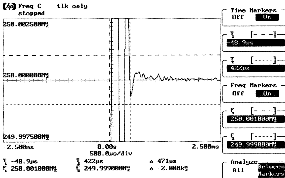
Positive Lock Time to within 1 kHz Range
