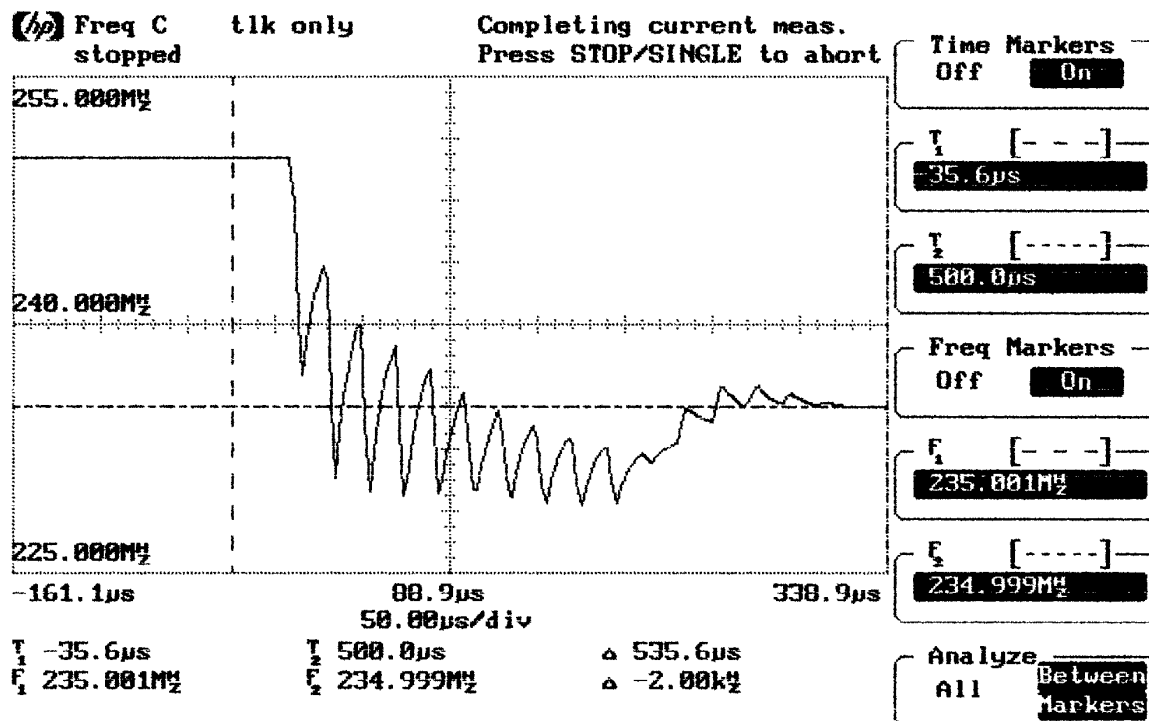
Negative Frequency Switching Waveform
