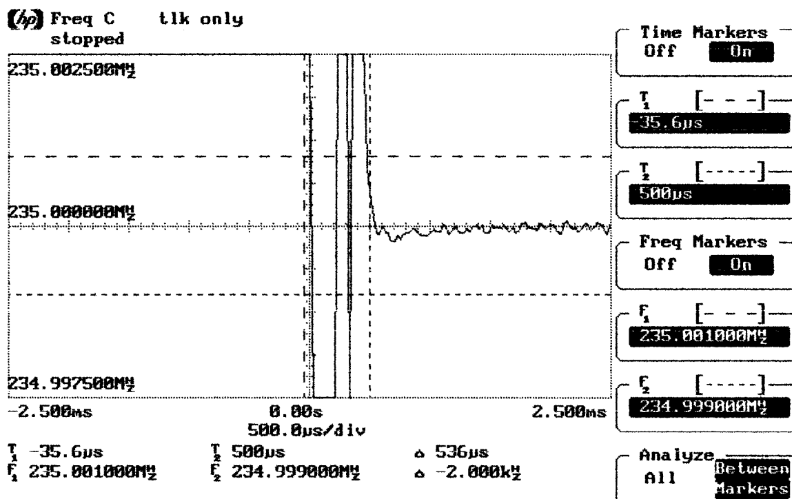
Negative Lock Time to within 1kHz Range
