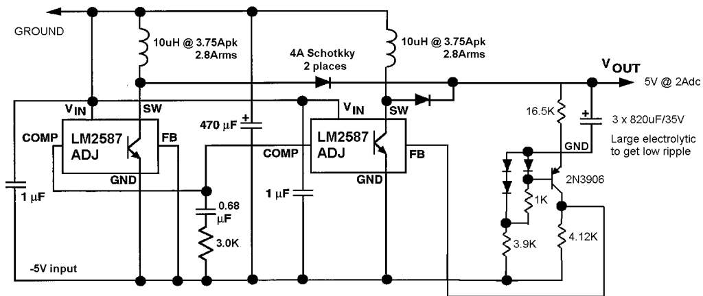
DUAL LM2587 BOOST CIRCUIT
