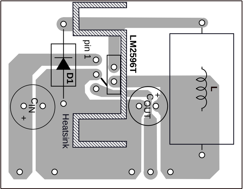
Component Side
