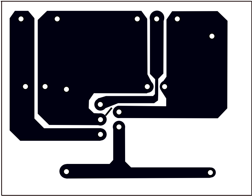
Copper side
