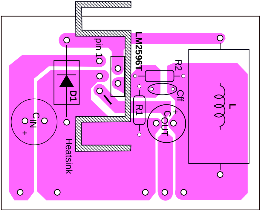
Component Side
