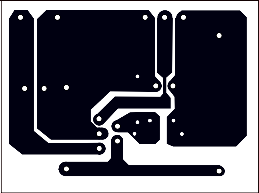
Copper side
