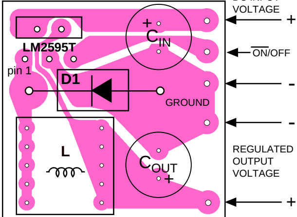
Component Side
