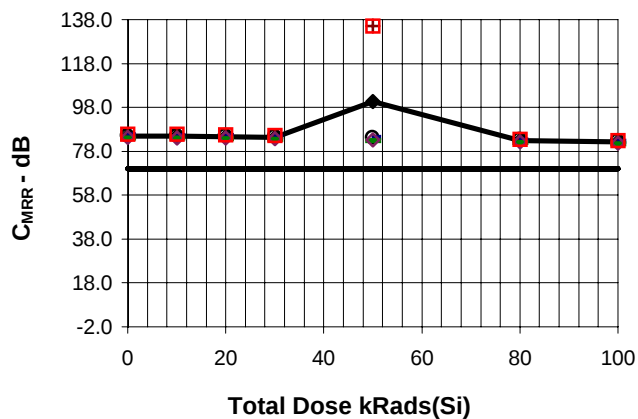
C_{MRR} ; V_+=30V , V_I=0-28V , AMP 2 vs Total Dose
