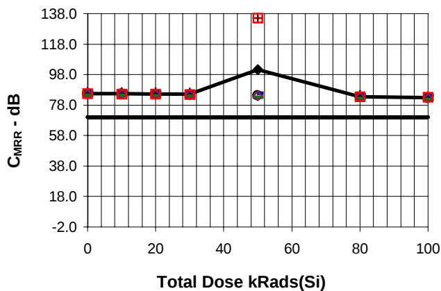
C_{MRR} ; V_+=30V , V_I=0-28V , AMP 1 vs Total Dose
