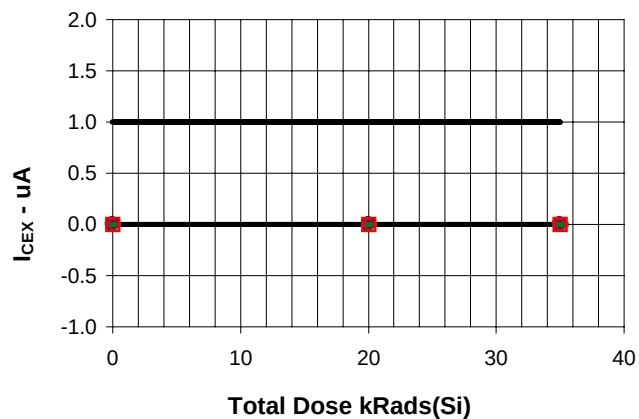
I_{CEX} ; V+=30V , COMP 1 vs Total Dose
