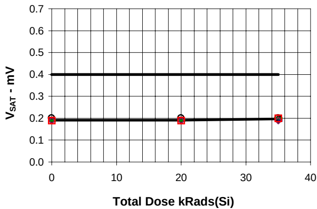
V_{SAT} ; I_{SINK}=4ma , COMP 1 vs Total Dose
