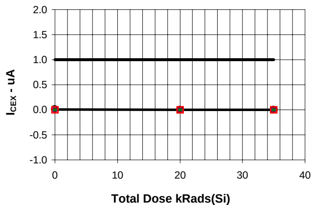
I_{CEX} ; V+=30V , COMP 2 vs Total Dose
