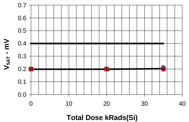
V_{SAT} ; I_{SINK}=4ma , COMP 2 vs Total Dose
