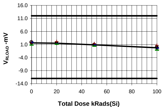
V_{RLOAD} ; V_I = 6.25\text{V} vs Total Dose
