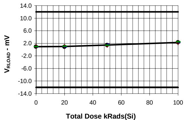
V_{RLOAD} ; V_I = 41.25\text{V} vs Total Dose
