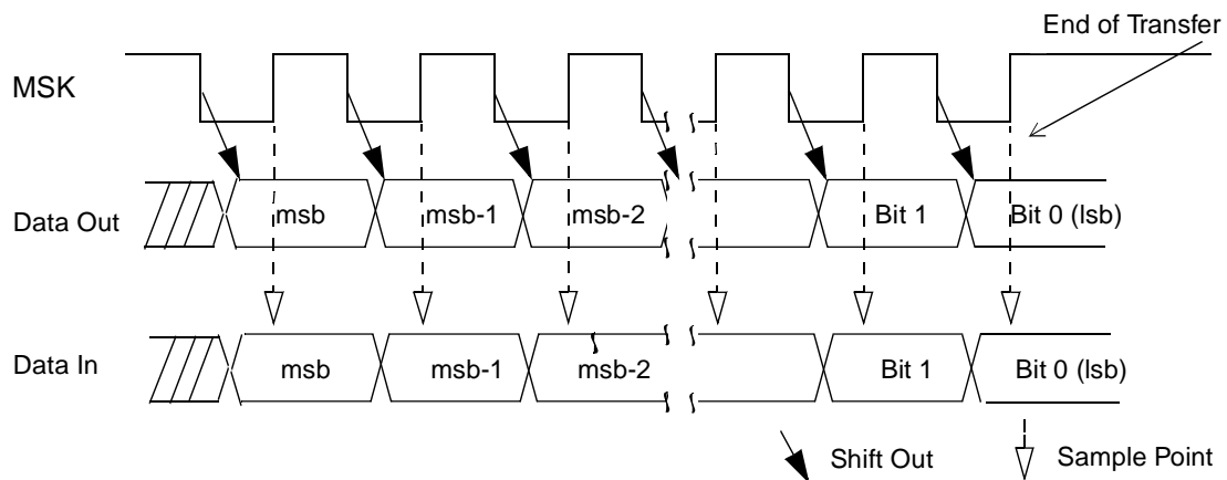
Figure 22. Normal Mode, MIDL Bit = 1
