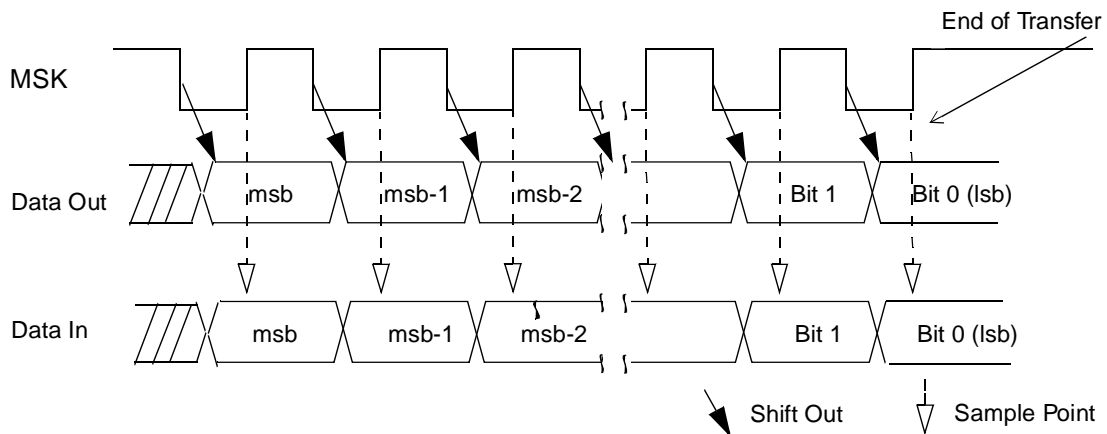
Figure 23. Alternate Mode, MIDL Bit = 0
