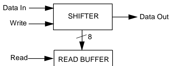
Figure 27. MWDAT Register Structure
