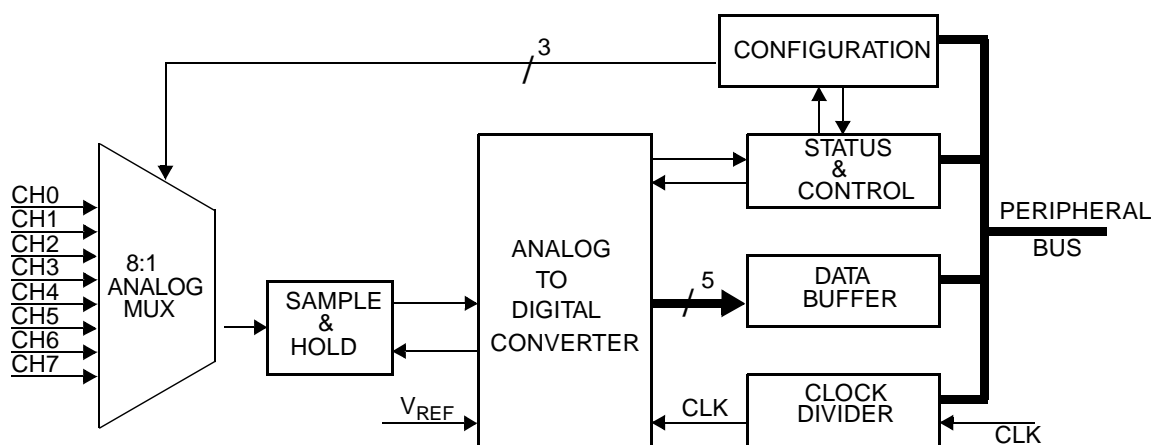
Figure 36. A/D Converter Block Diagram
