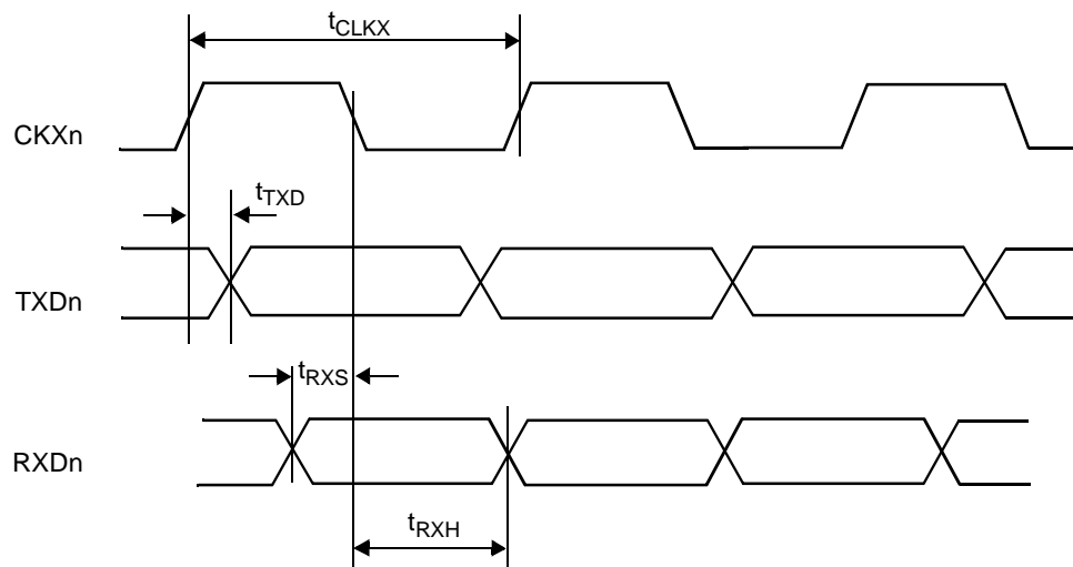
Figure 44. USART Synchronous Mode Timing
