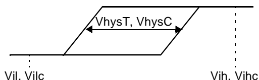
Figure 39. Hysteresis Input Definition
