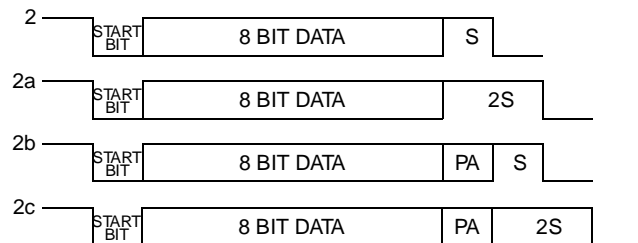
Figure 32. Eight Data Bit Frame Options
