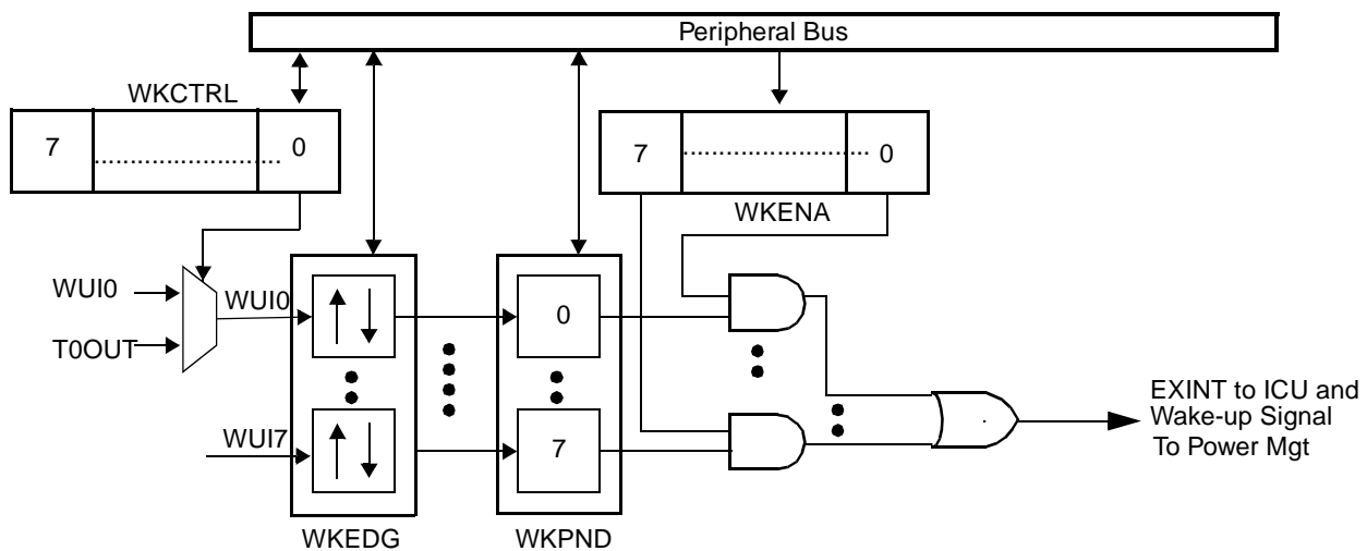
Figure 10. Multi-Input Wake-Up Module Block Diagram
