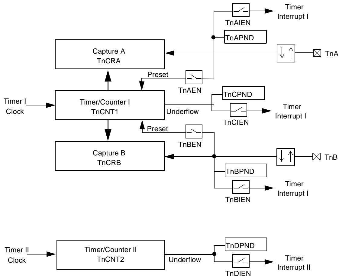
Figure 16. Mode 2: Dual Input Capture Block Diagram
