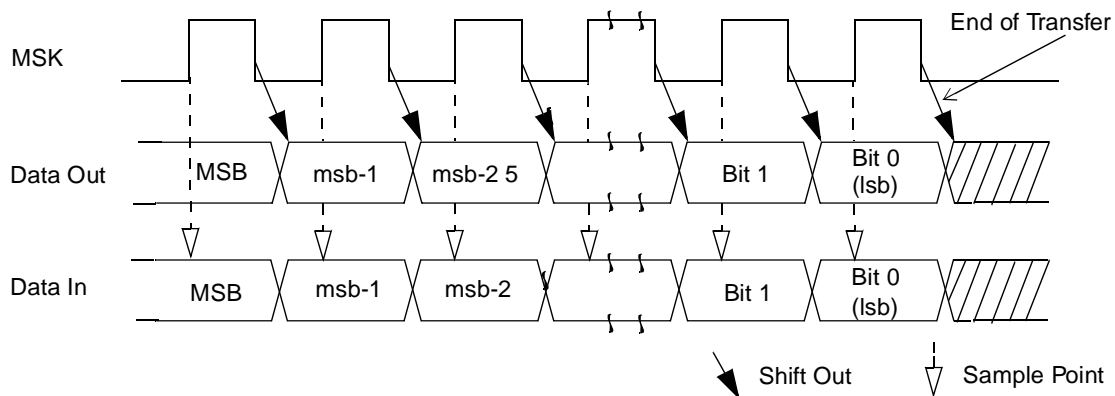
Figure 24. Alternate Mode, MIDL Bit = 1
