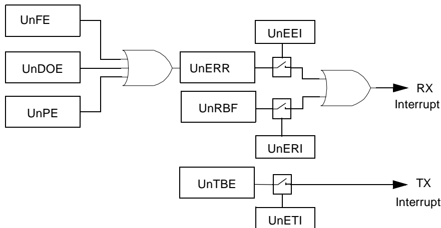
Figure 34. USART Interrupts
