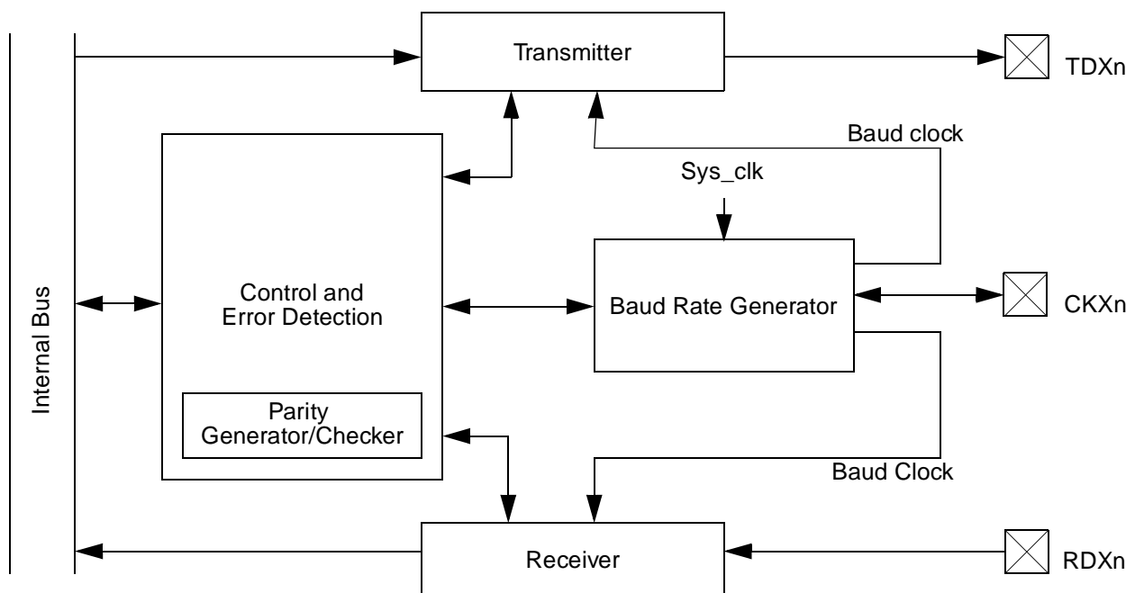
Figure 28. USART Block Diagram
