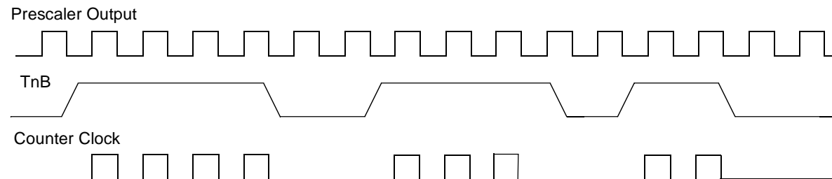
Figure 14. Pulse Accumulate Mode Operation
