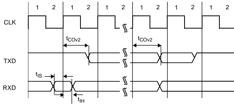
Figure 43. USART Asynchronous Mode Timing
