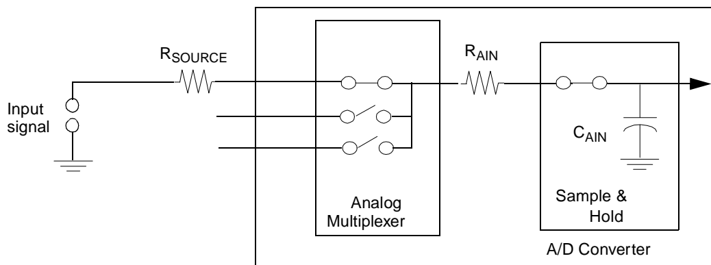
Figure 37. Sample-and-Hold Charge-Up Schematic
