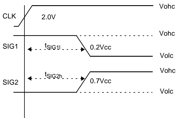
Figure 38. CMOS Output Signal Specification Standard
