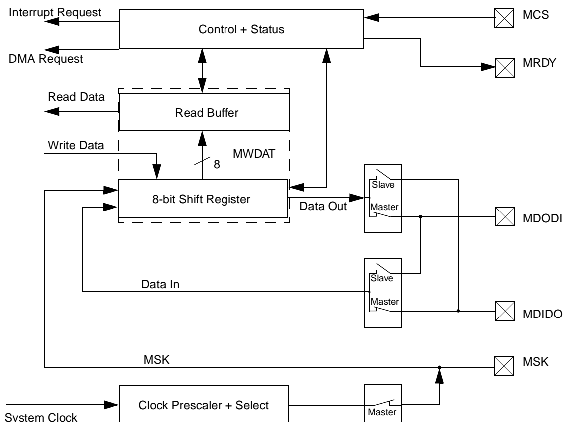
Figure 20. MICROWIRE Block Diagram
