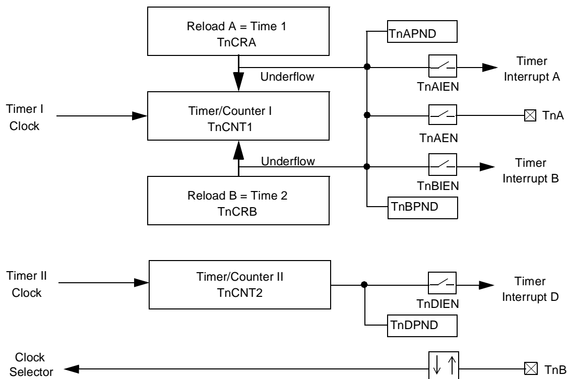
Figure 15. Mode 1: Processor-Independent PWM Block Diagram
