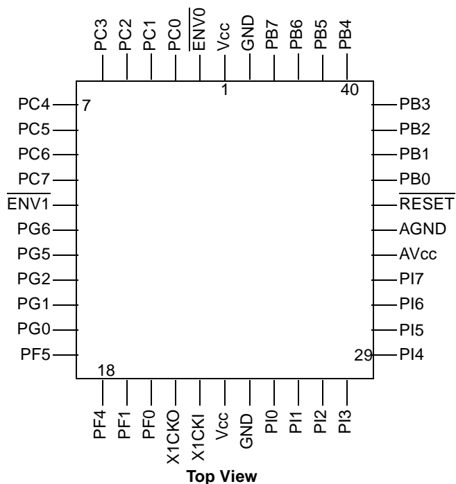
Order Number CR16MES944V7 See NS Package Number V44A Figure 1.
