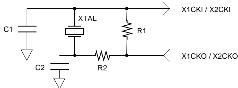
Figure 9. External Crystal Network
