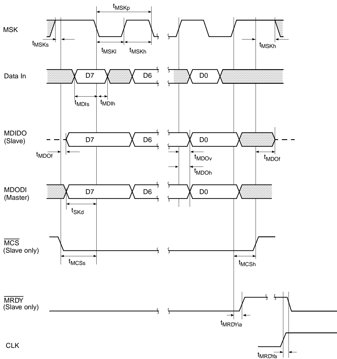
Figure 49. MICROWIRE Transaction Timing, Alternate Mode, MIDL bit = 1
