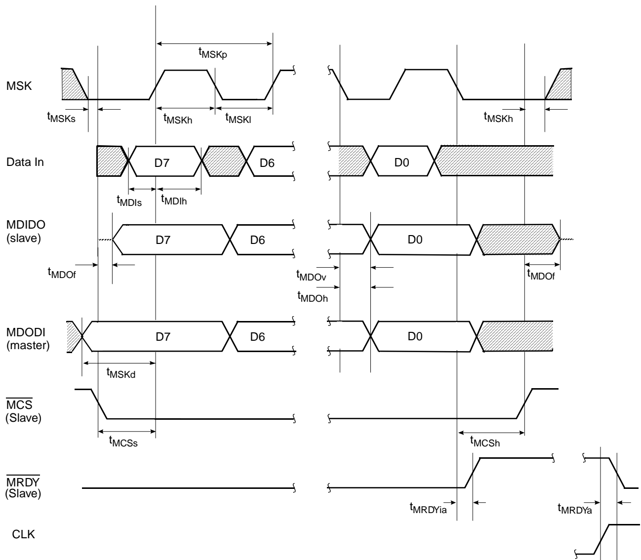
Figure 48. MICROWIRE Transaction Timing, Alternate Mode, MIDL bit = 0
