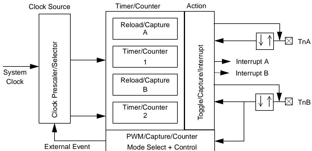
Figure 12. Multi-Function Timer Block Diagram
