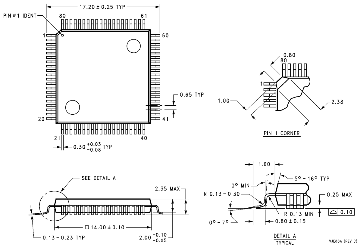
80 Lead Molded Plastic Quad Flat Package Order Number CR16MHS9VJE7 See NS Package Number VJE80A
