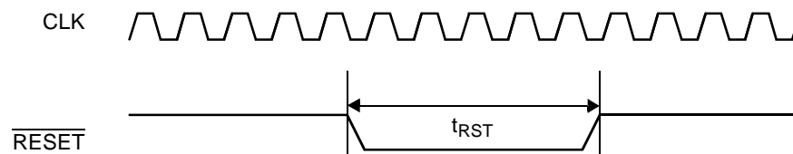
Figure 42. Non-Power-On Reset
