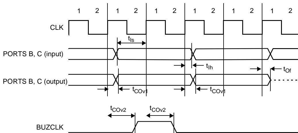
Figure 45. Ports Signals Timing
