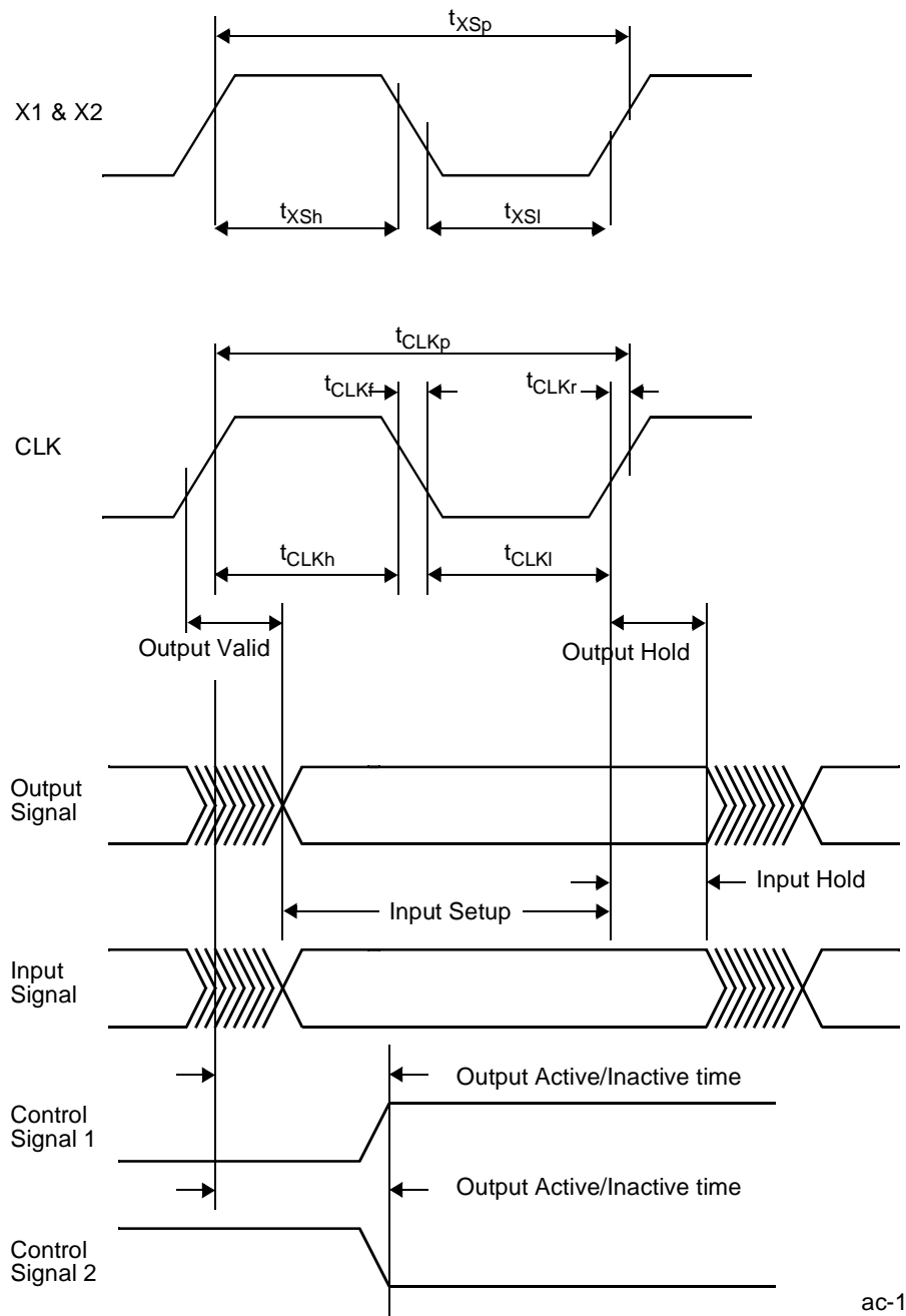
Figure 40. Clock Waveforms
