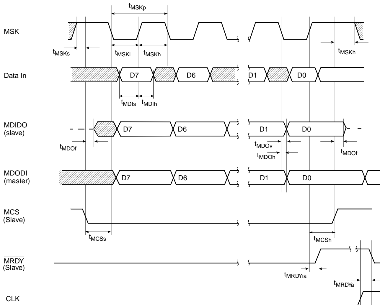
Figure 46. MICROWIRE Transaction Timing, Normal Mode, MIDL Bit = 0
