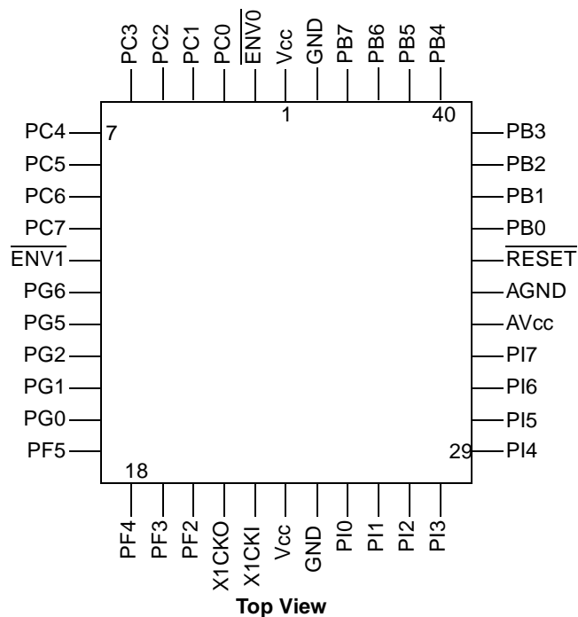
Order Number CR16MFS944V7 See NS Package Number V44A Figure 2.
