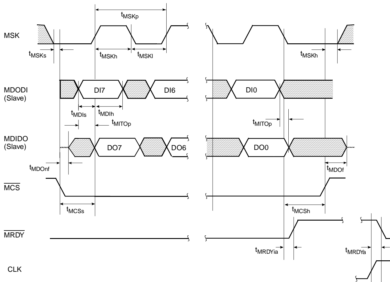
Figure 50. MICROWIRE Transaction Timing, Data Echoed to Output, Normal Mode, MIDL Bit = 0, MECH Bit = 1, Slave
