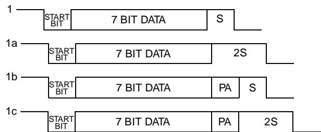
Figure 31. Seven Data Bit Frame Options
