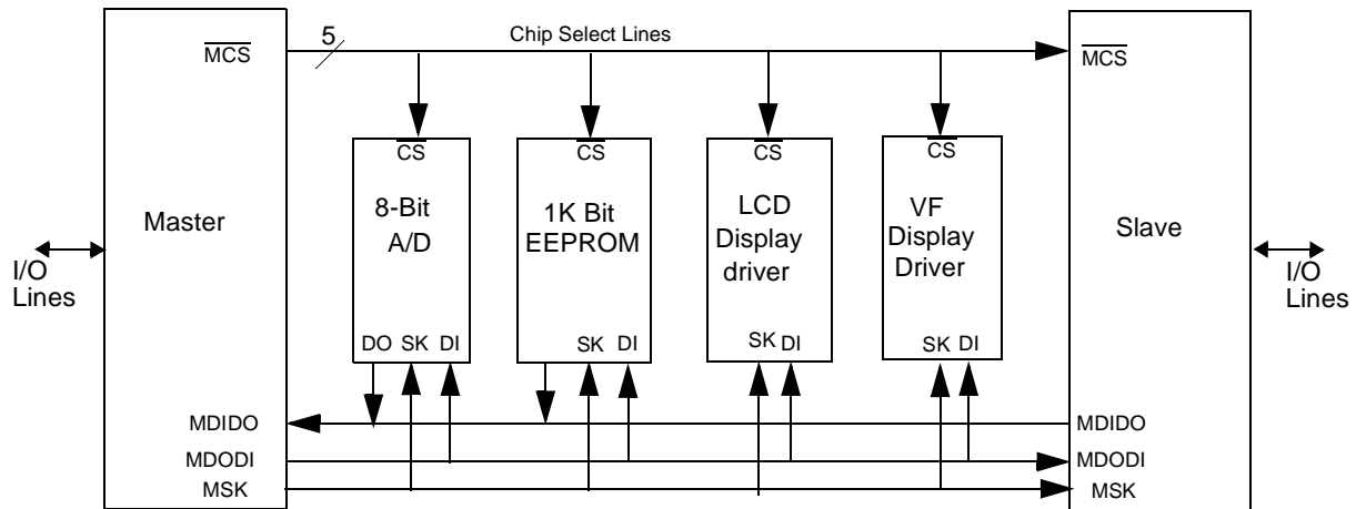
Figure 19. MICROWIRE Interface
