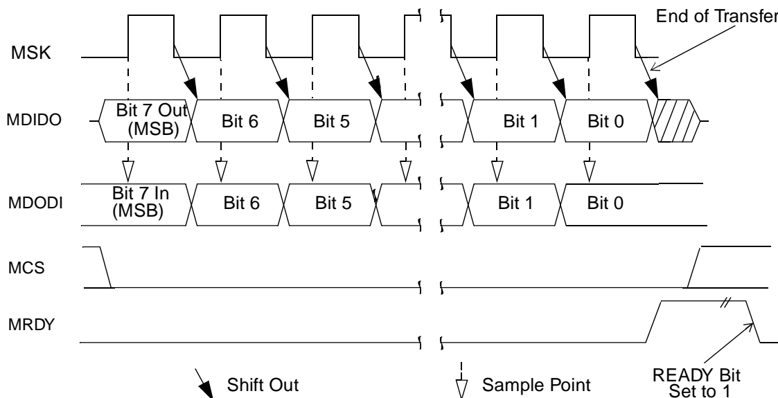
Figure 25. Slave, Normal Mode, MIDL Bit = 0, MRBF Bit = 1
