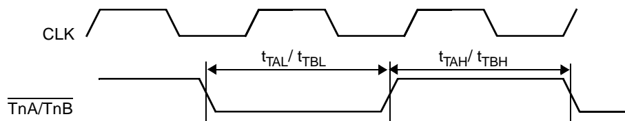
Figure 51. Multi-Function-Timer (MFT16) Input Timing
