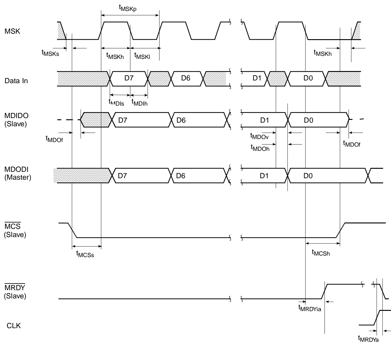
Figure 47. MICROWIRE Transaction Timing, Normal Mode, MIDL bit = 1
