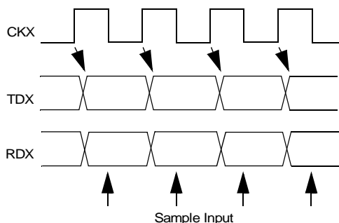
Figure 30. USART Synchronous Communication
