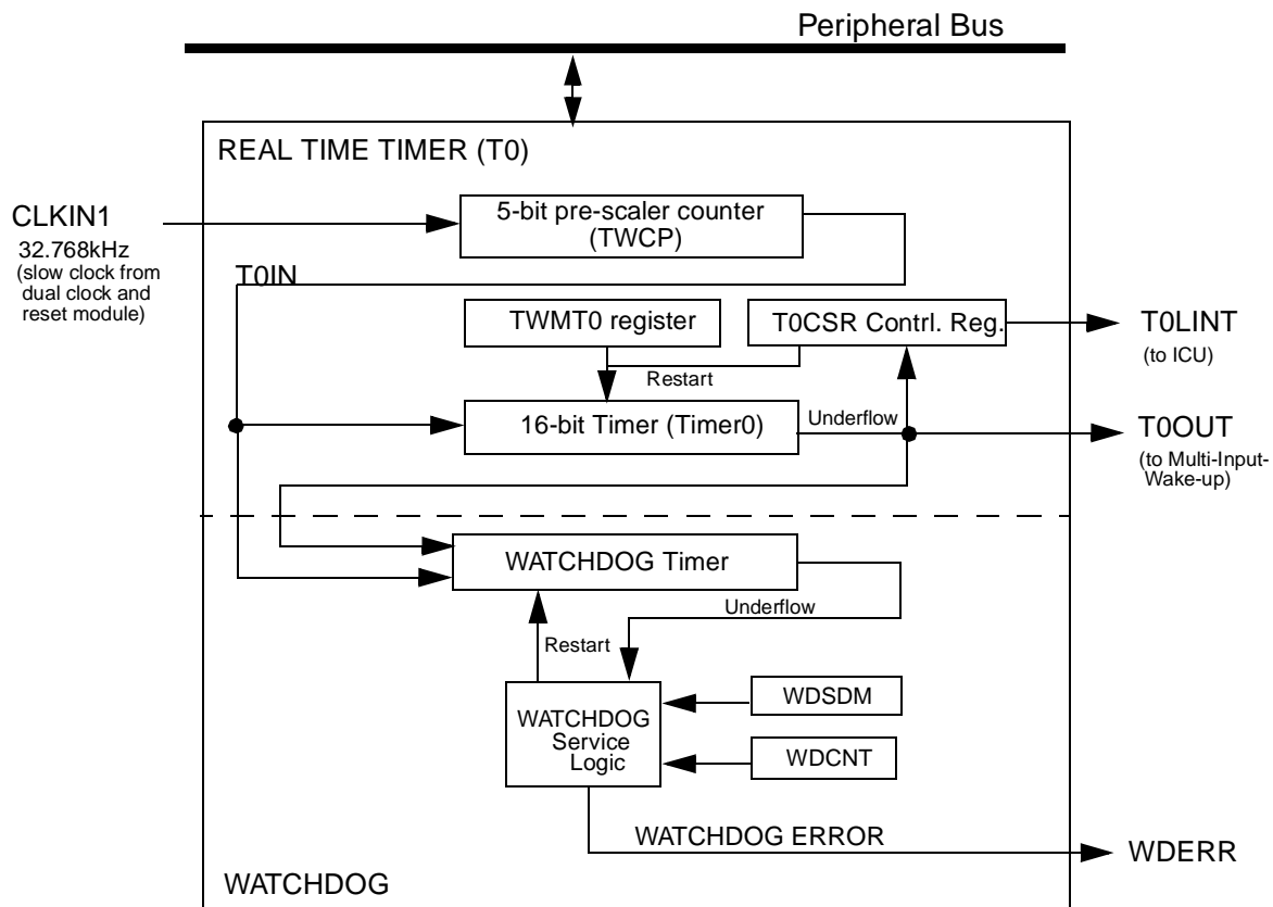
Figure 11. Timing and WATCHDOG Module Block Diagram
