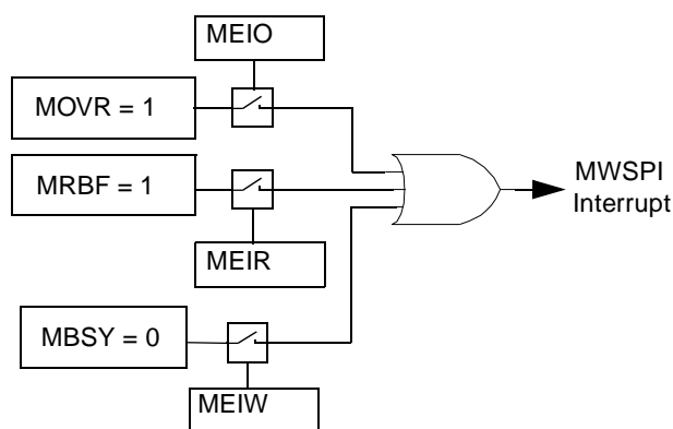
Figure 26. MWSPI Interrupts
