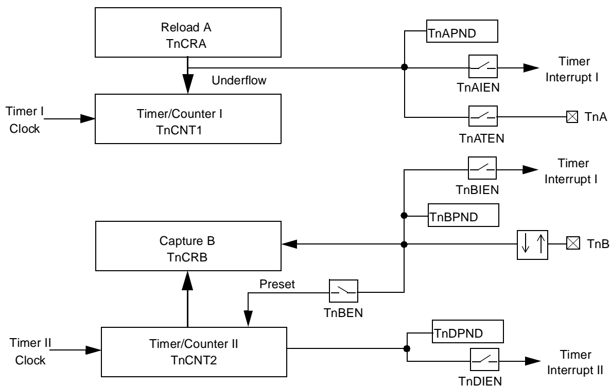
Figure 18. Mode 4: Input Capture Plus Timer Block Diagram
