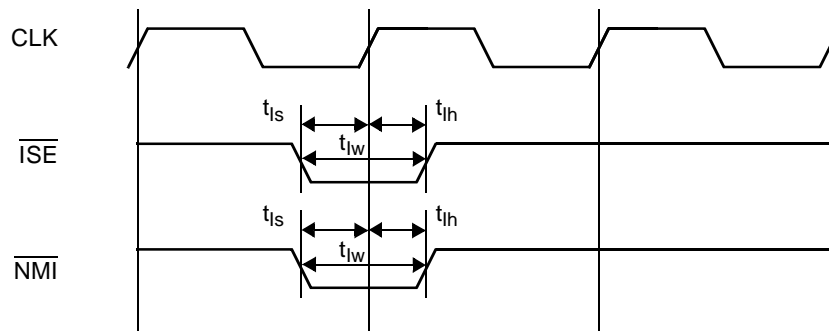
Figure 41. ISE & NMI Signal Timing
