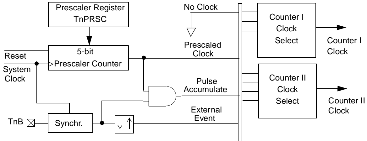
Figure 13. Clock Source Block Diagram
