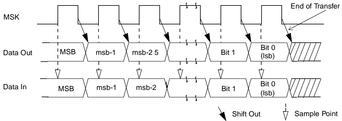
Figure 21. Normal Mode, MIDL Bit = 0
