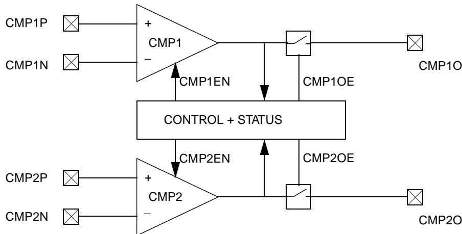
Figure 35. Dual Analog Comparator Block Diagram
