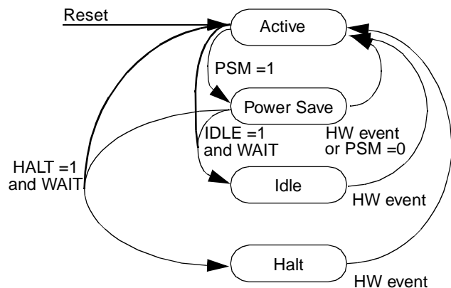
Figure 7. Power Modes and Transitions
