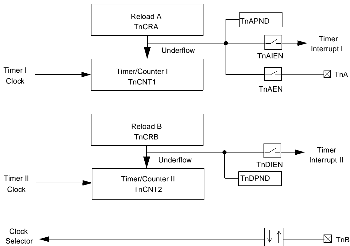
Figure 17. Mode 3: Dual Independent Timer/Counter Block Diagram
