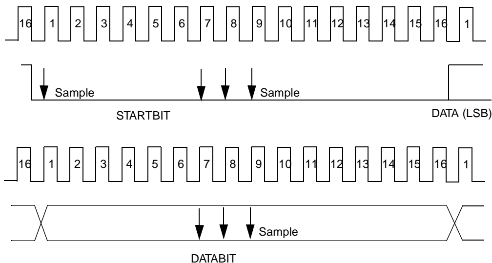
Figure 29. USART Asynchronous Communication
