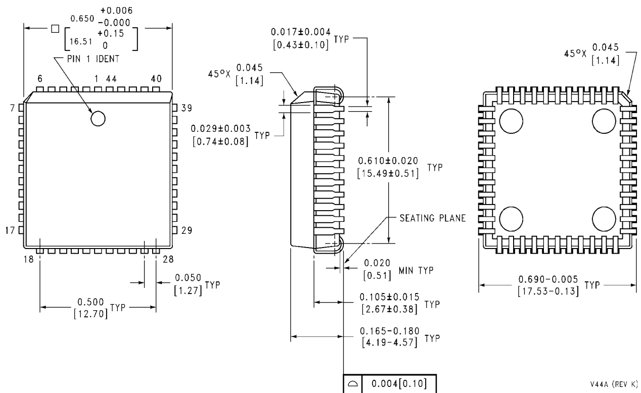
44 Lead Molded Plastic Leaded Chip Carrier Order Number CR16MES944V7 or CR16MFS944V7 See NS Package Number V44A
