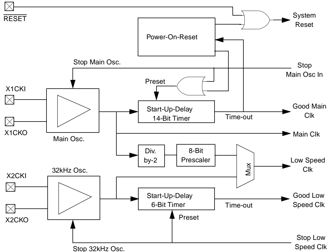
Figure 8. Dual Clock and Reset Module Block Diagram
