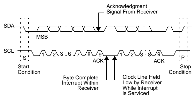
Figure 42. ACCESS.bus Data Transaction
