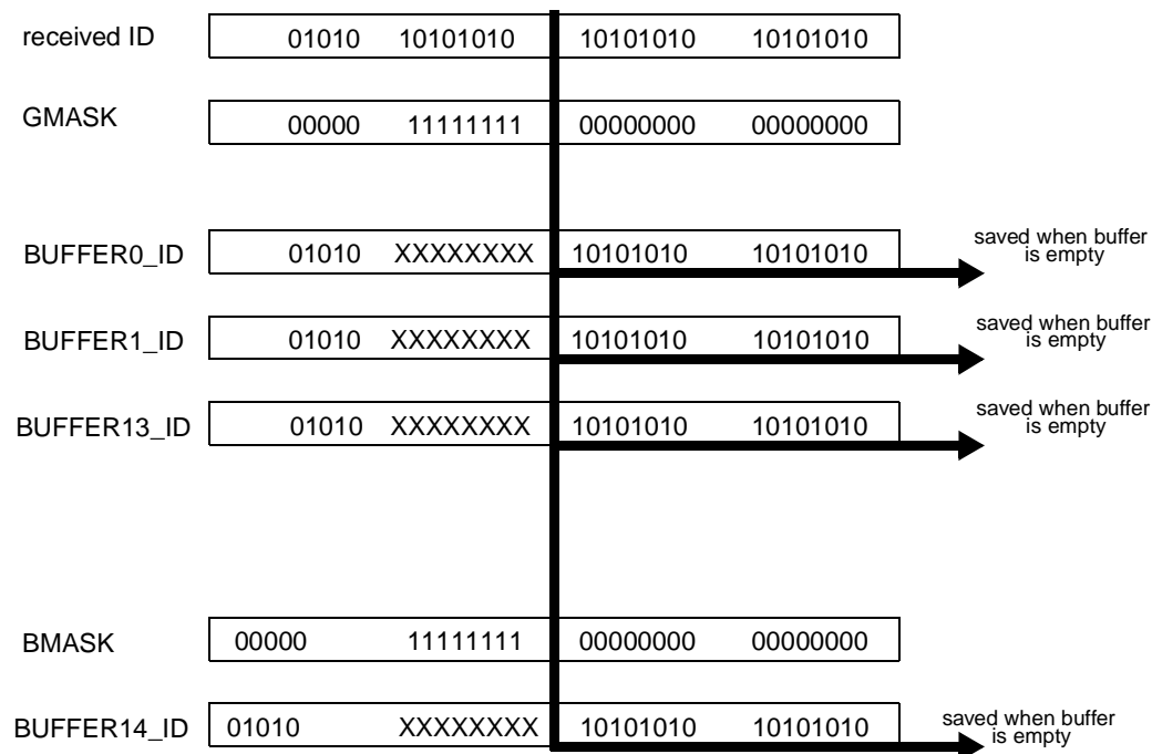
Figure 60. Message Storage with BUFFLOCK Enabled
