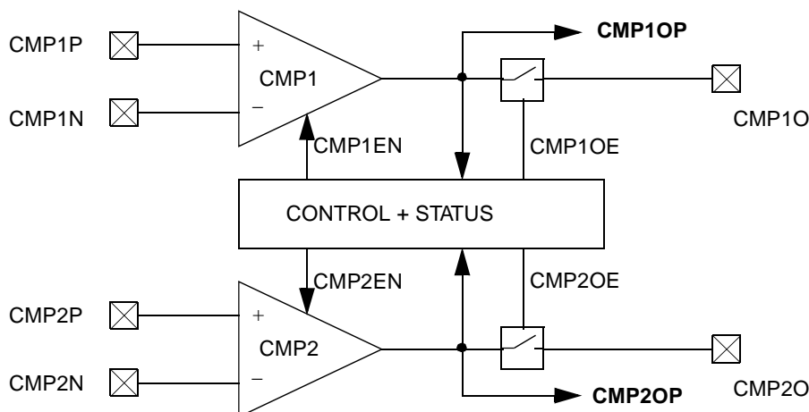
Figure 74. Dual Analog Comparator Block Diagram
