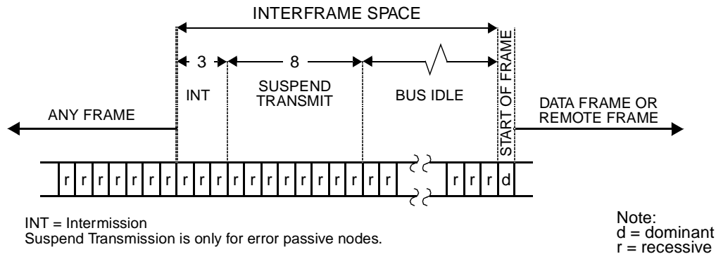
Figure 51. CAN Interframe Space
