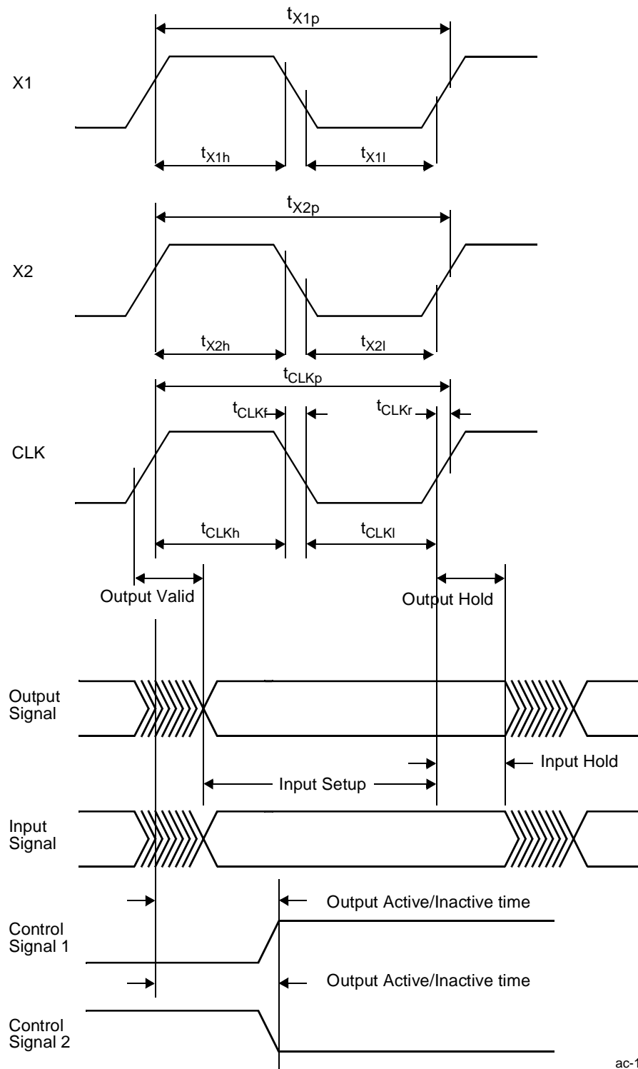
Figure 79. Clock Waveforms
