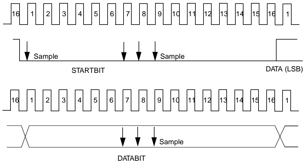
Figure 34. USART Asynchronous Communication
