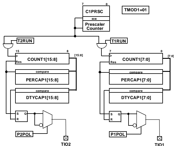
Figure 21. VTU Dual 8-bit PWM Mode
