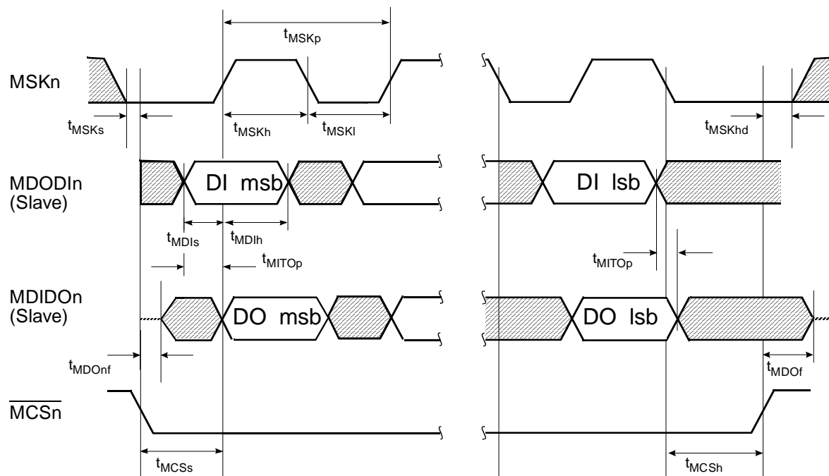
Figure 89. MICROWIRE Transaction Timing, Data Echoed to Output, Normal Mode, MIDL Bit = 0, MECH Bit = 1, Slave
