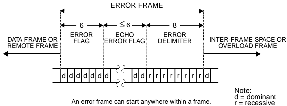
Figure 49. CAN Error Frame
