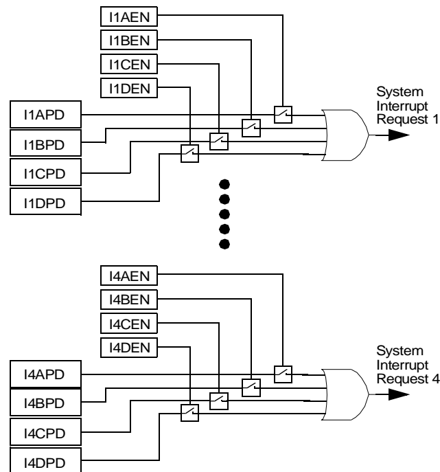
Figure 24. VTU Interrupt Request Structure
