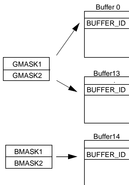
Figure 57. Acceptance Filtering Structure
