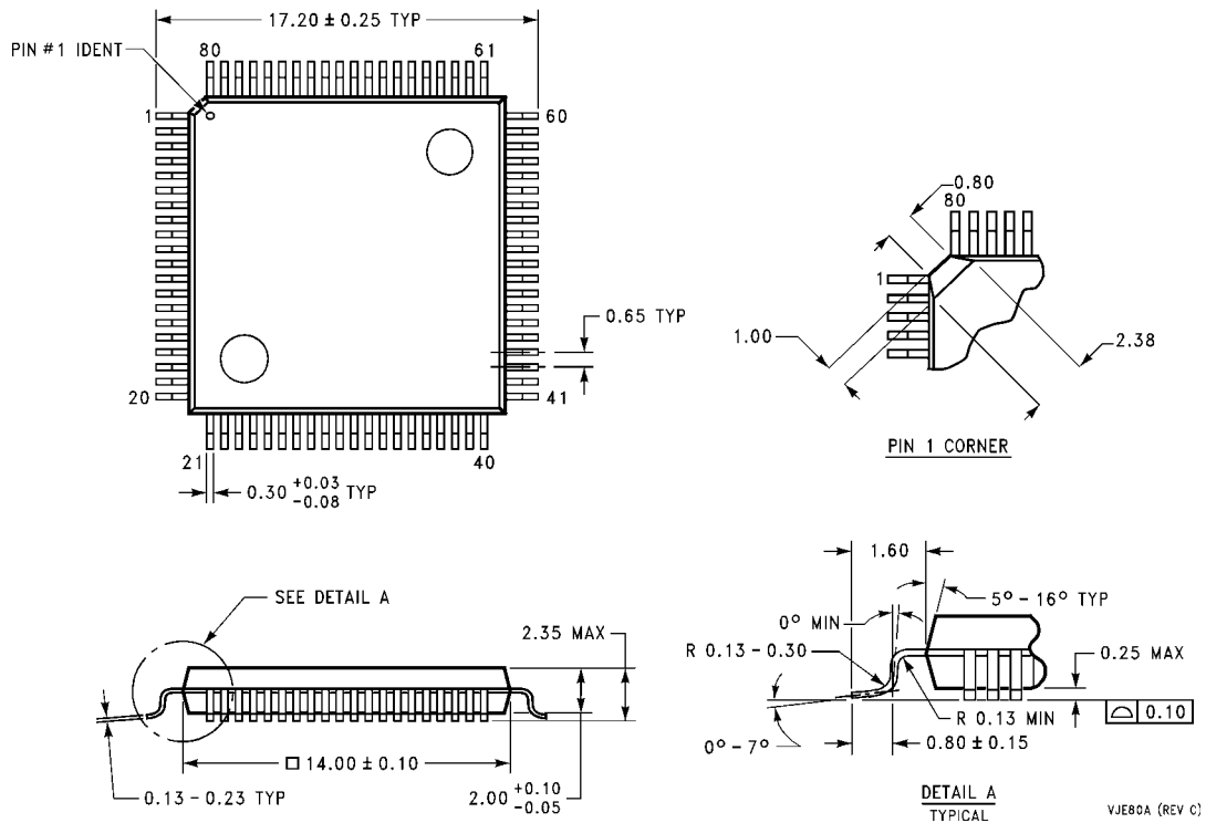
80 Lead Molded Plastic Quad Flat Package Order Number CR16MCS9VJE7 See NS Package Number VJE80A
