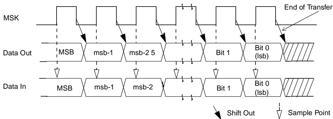
Figure 30. Alternate Mode, MIDL Bit = 1
