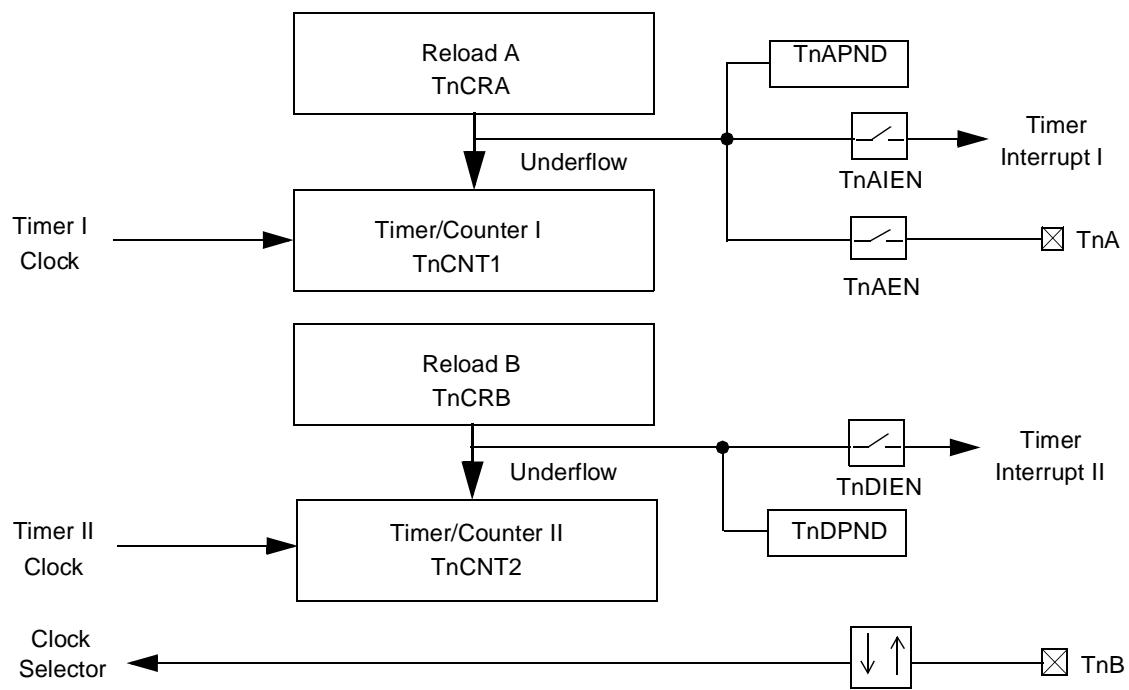
Figure 17. Mode 3: Dual Independent Timer/Counter Block Diagram
