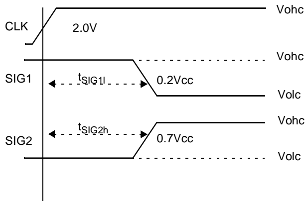
Figure 77. CMOS Output Signal Specification Standard
