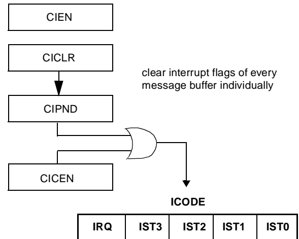
Figure 68. CR16CAN Interrupt Management
