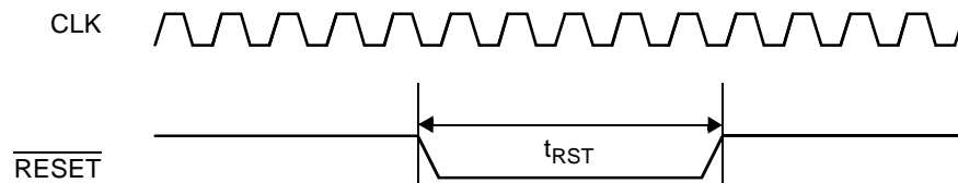
Figure 81. Non-Power-On Reset
