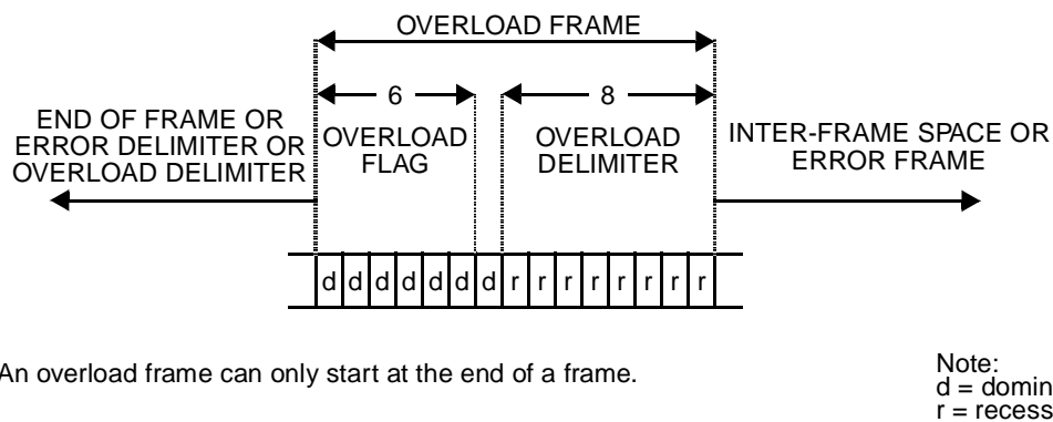
Figure 50. CAN Overload Frame
