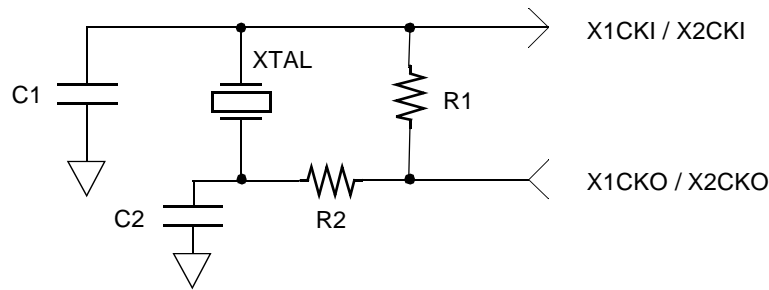
Figure 9. External Crystal Network
