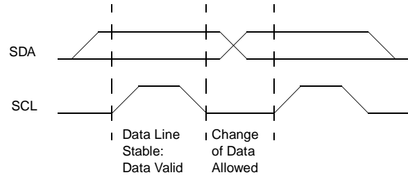
Figure 40. Bit Transfer
