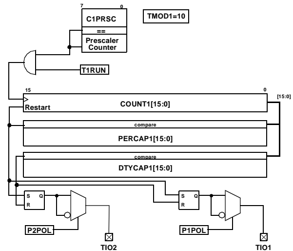
Figure 22. VTU 16-bit PWM Mode
