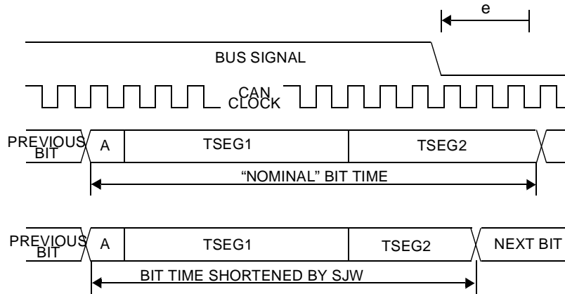
Figure 55. Re-synchronization ( e < -SJW )
