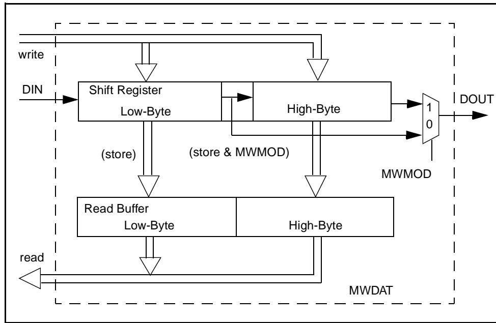
Figure 32. MWDAT Register Structure
