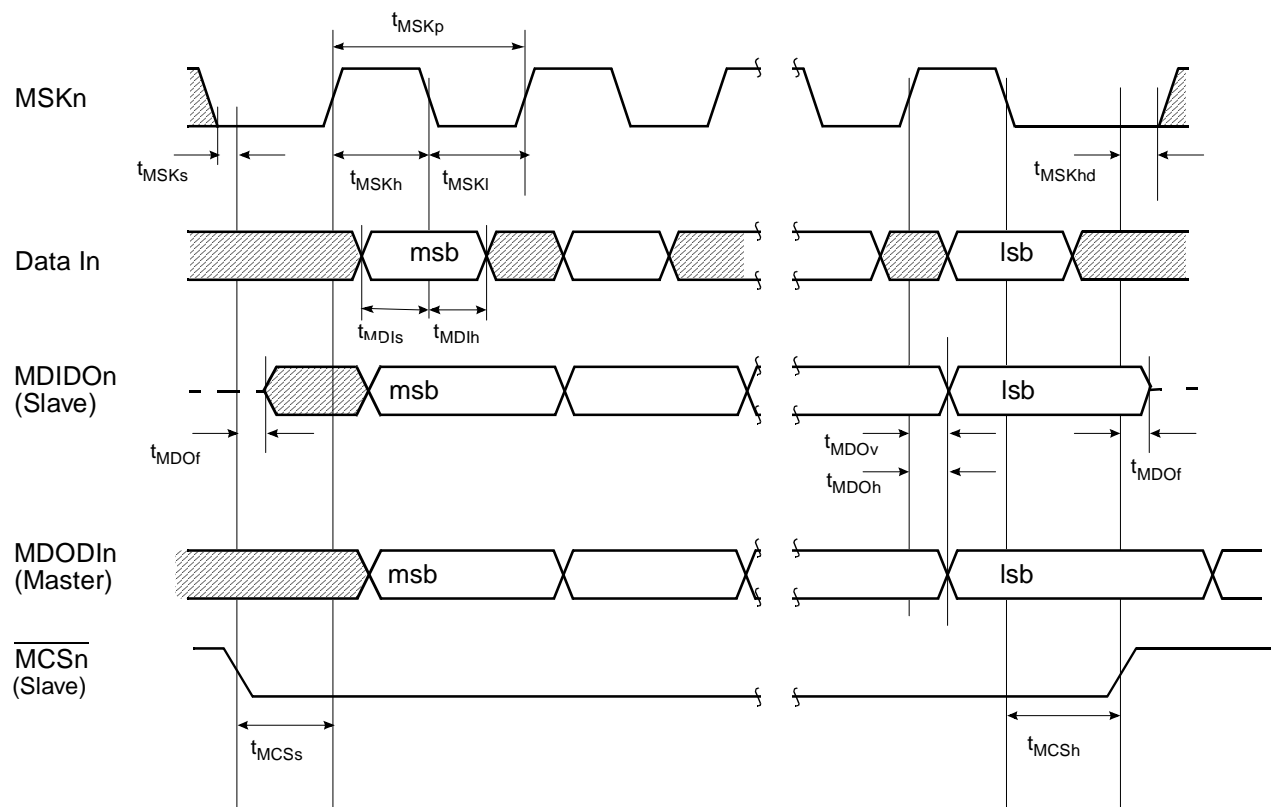
Figure 87. MICROWIRE Transaction Timing, Alternate Mode, MIDL bit = 0
