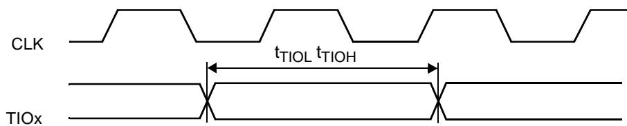
Figure 94. Versatile-Timer-Unit Input Timing
