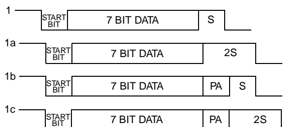
Figure 36. Seven Data Bit Frame Options
