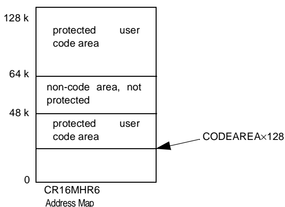
Figure 3. Memory Protection through CODEAREA
