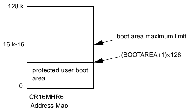
Figure 4. Memory Protection through BOOTAREA
