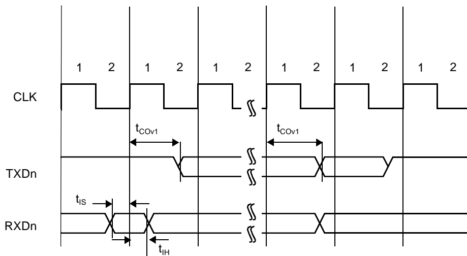
Figure 82. USART Asynchronous Mode Timing
