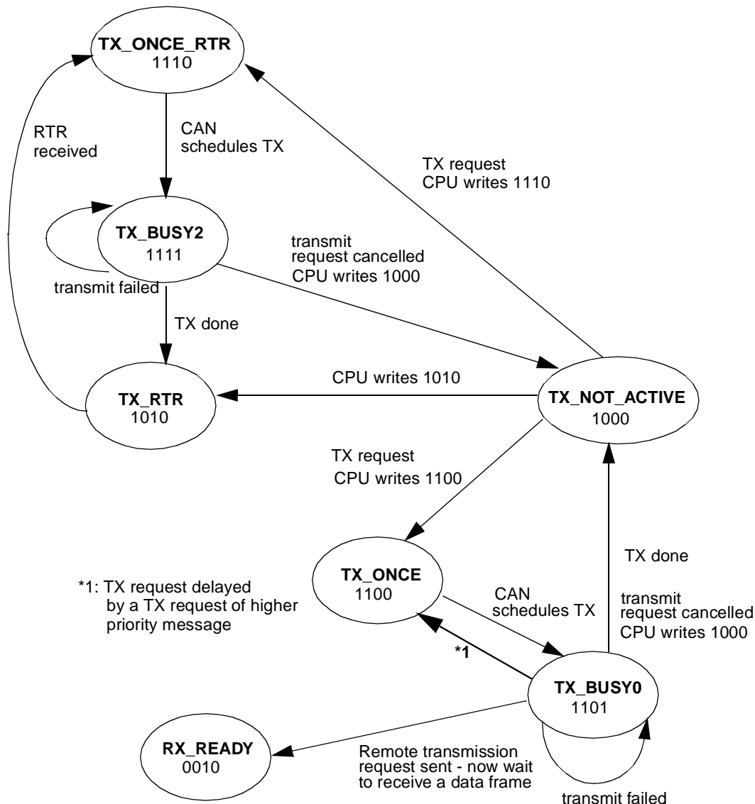
Figure 67. Transmit Buffer States
