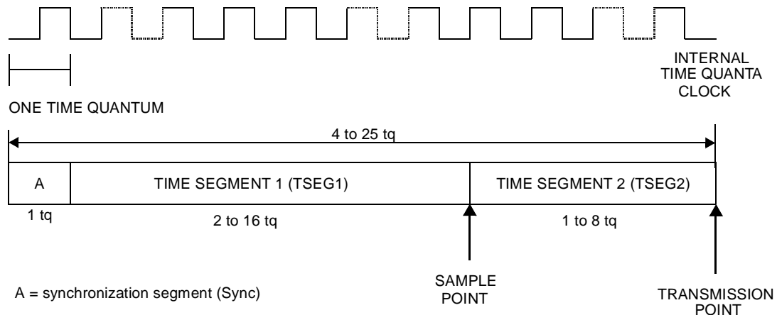
Figure 53. Bit Timing
