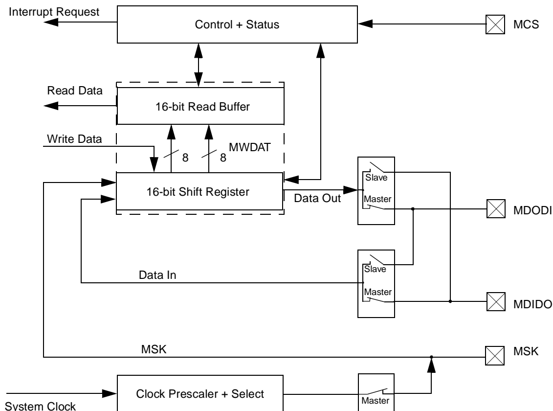
Figure 26. MICROWIRE Block Diagram
