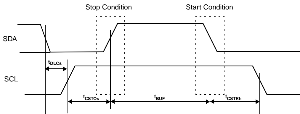
Figure 91. ACB Start and Stop Condition Timing
