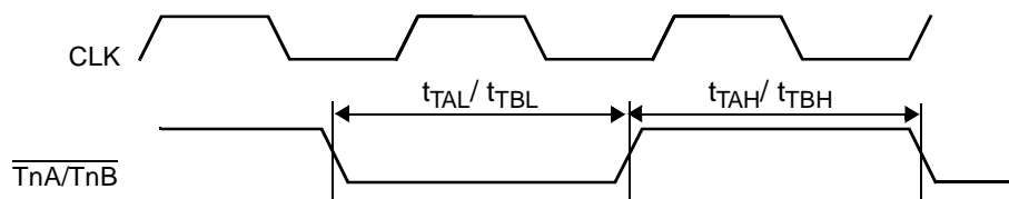
Figure 93. Multi-Function-Timer (MFT16) Input Timing
