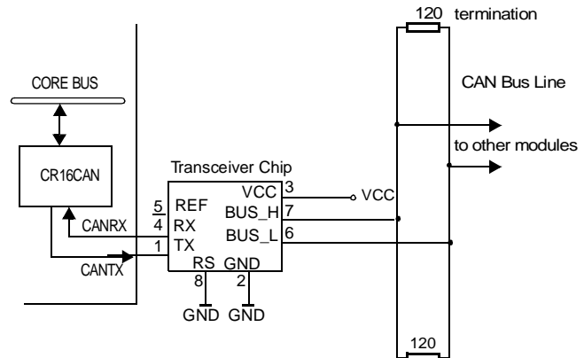
Figure 73. External Transceiver Connection (ISO-High-Speed)
