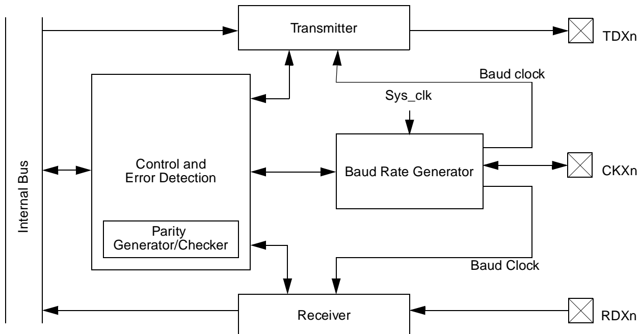
Figure 33. USART Block Diagram
