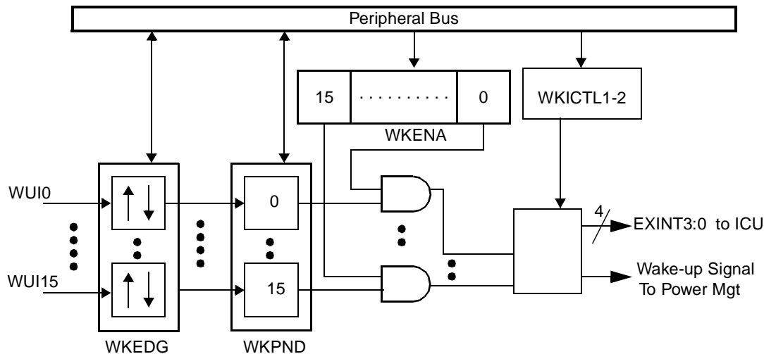
Figure 10. Multi-Input Wake-Up Module Block Diagram
