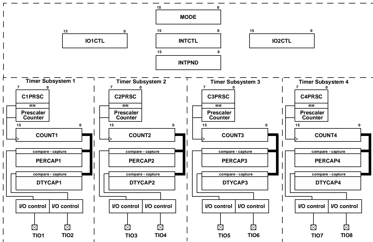
Figure 19. VTU Block Diagram
