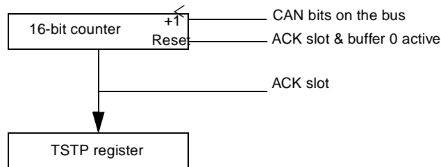
Figure 69. Time Stamp Counter
