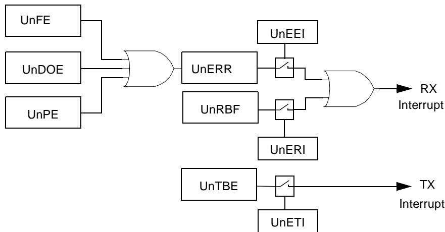
Figure 39. USART Interrupts
