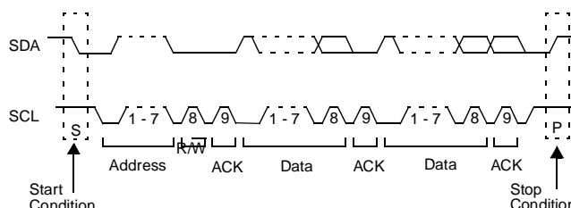
Figure 44. A Complete ACCESS.bus Data Transaction
