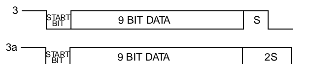
Figure 38. Nine Data Bit Frame Options
