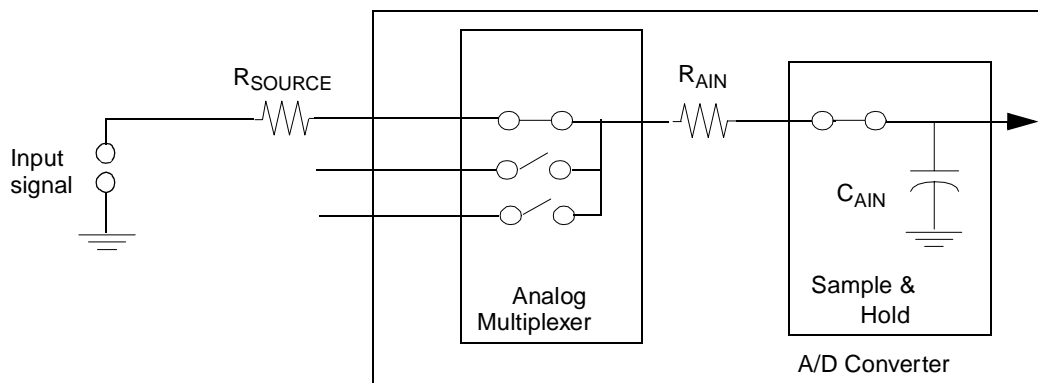
Figure 76. Sample-and-Hold Charge-Up Schematic
