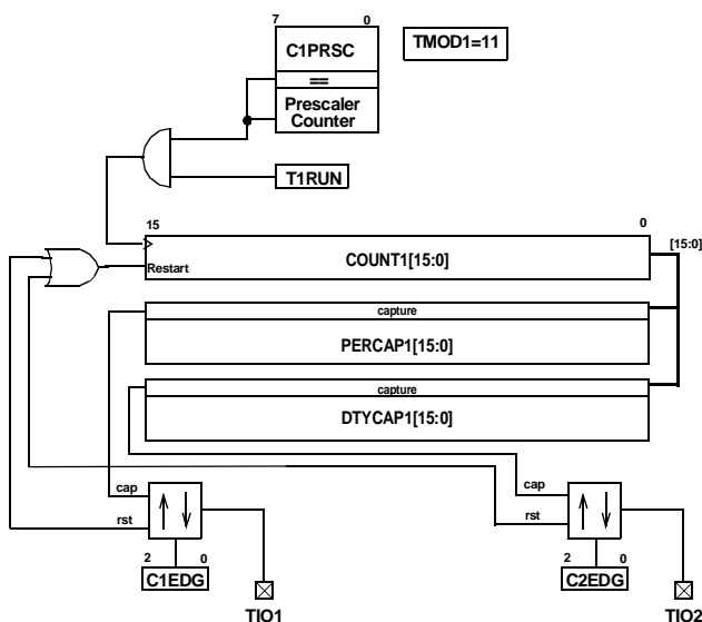
Figure 23. VTU Dual 16-bit Capture Mode
