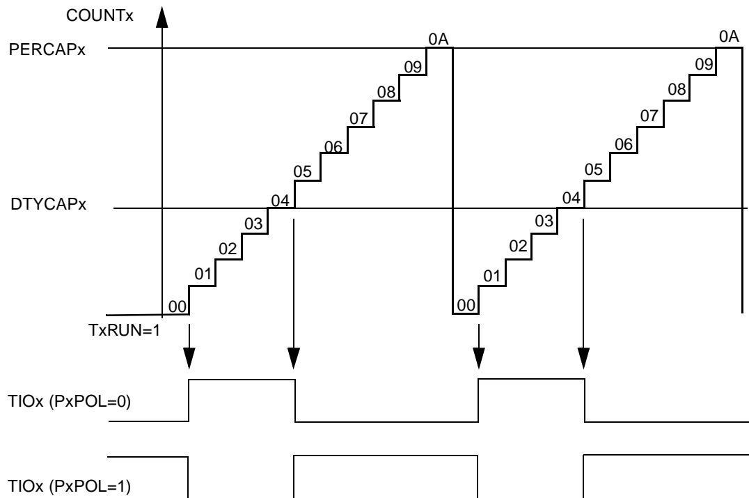
Figure 20. VTU PWM generation
