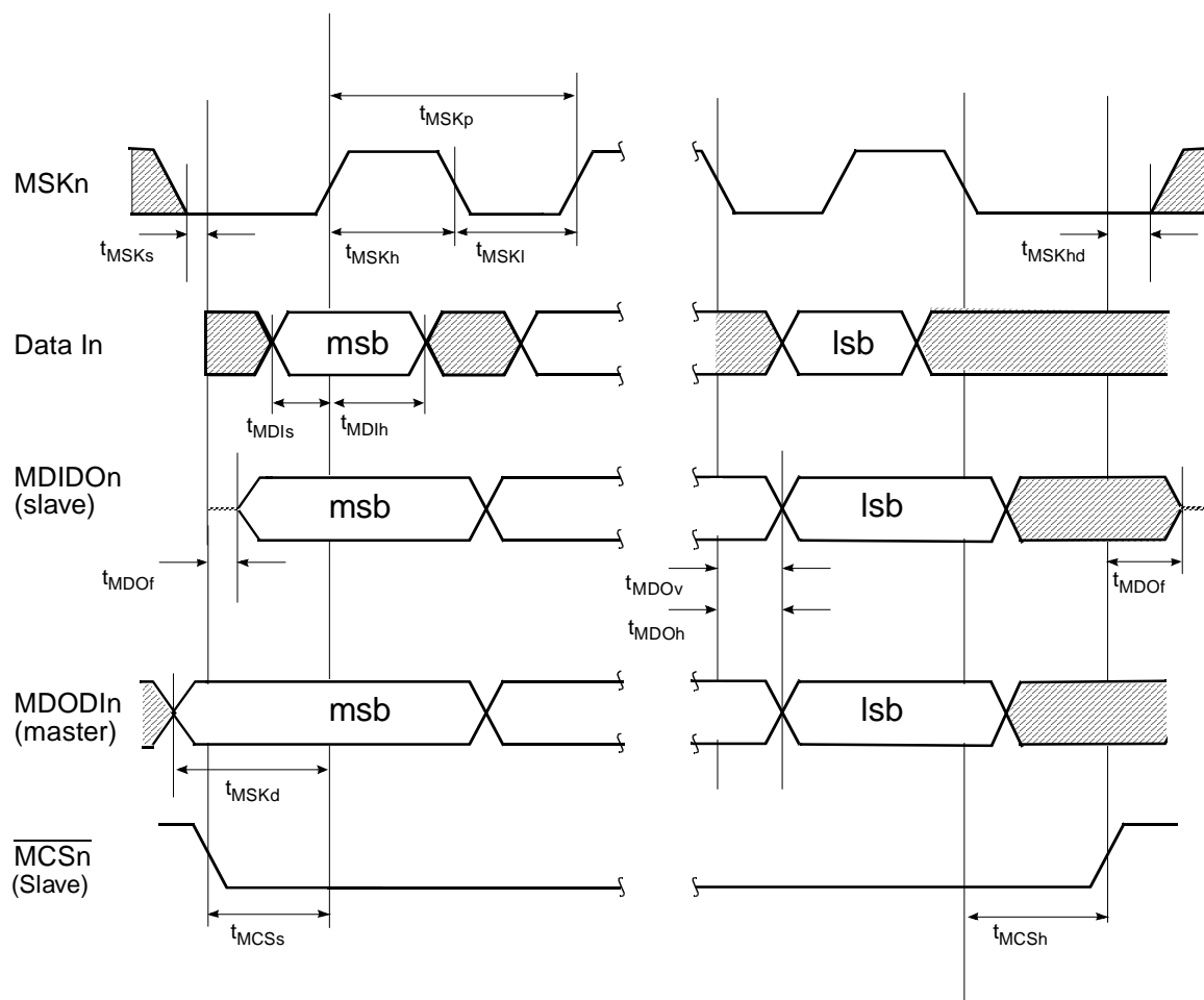
Figure 85. MICROWIRE Transaction Timing, Normal Mode, MIDL Bit = 0
