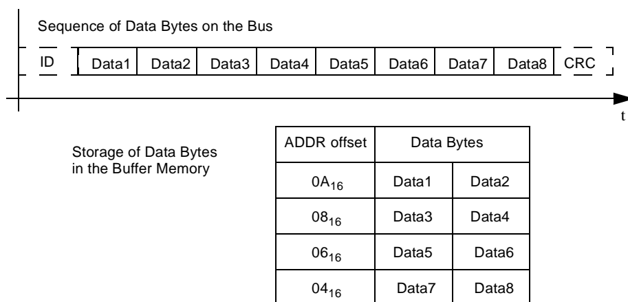
Figure 70. Data Direction Bit set to '0'
