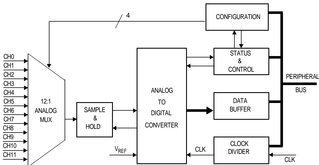
Figure 75. A/D Converter Block Diagram
