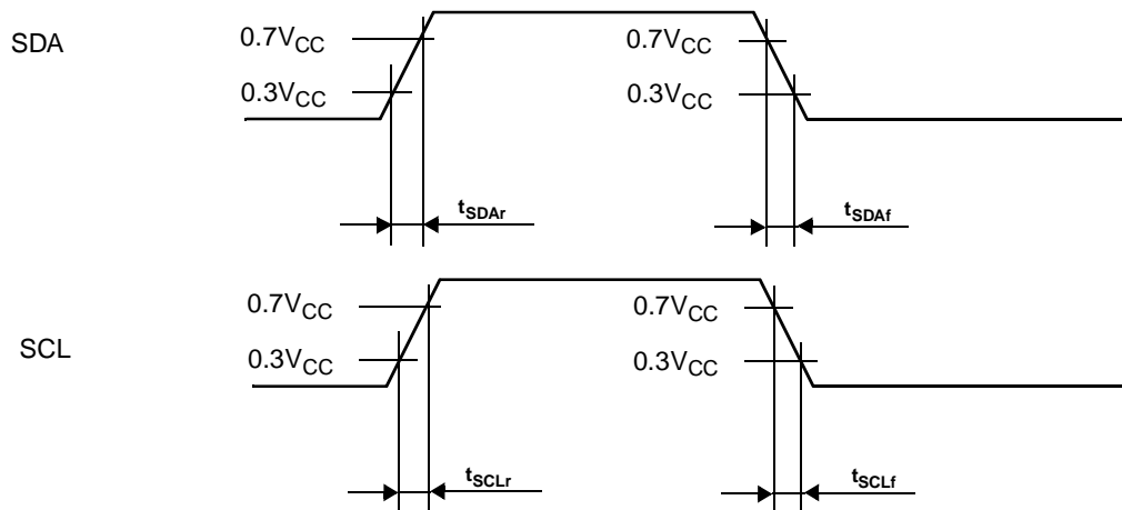
Figure 90. ACB signals (SDA and SCL) Rise Time and Fall Timing
