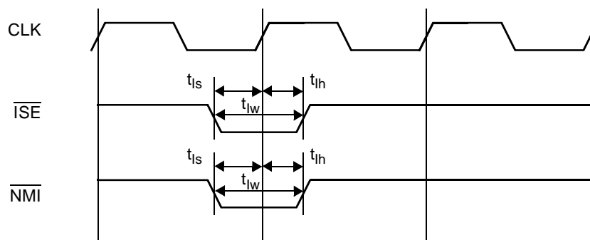
Figure 80. ISE & \overline{\text{NMI}} Signal Timing
