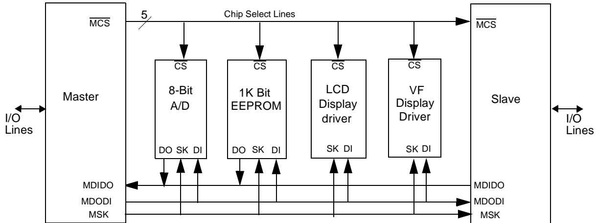
Figure 25. MICROWIRE Interface
