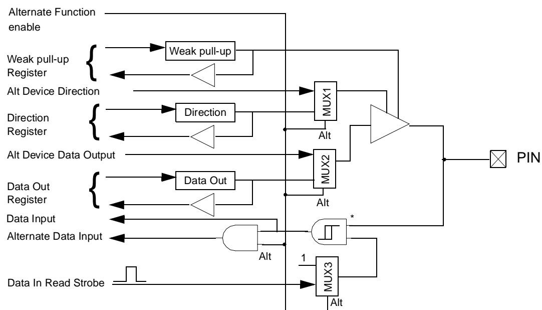
Figure 2. I/O Pin Functional Diagram
