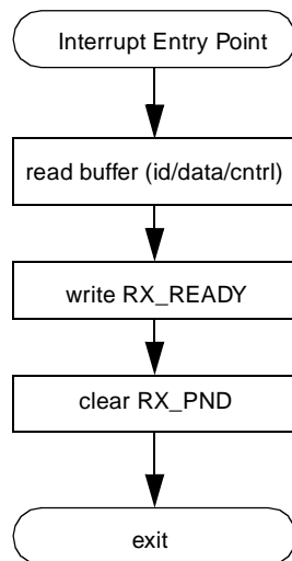
Figure 64. Buffer Read Routine (BUFFLOCK Enabled)
