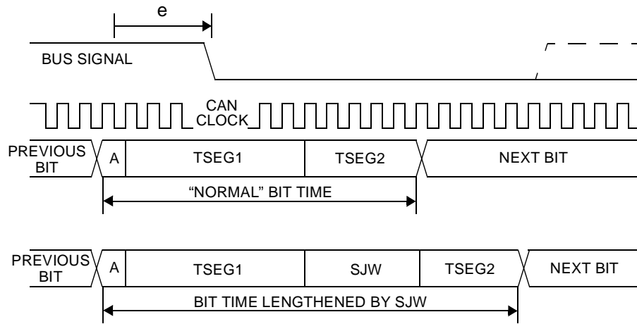
Figure 54. Re-synchronization ( e > SJW )
