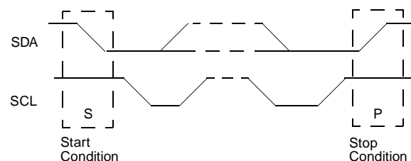
Figure 41. Start and Stop Conditions
