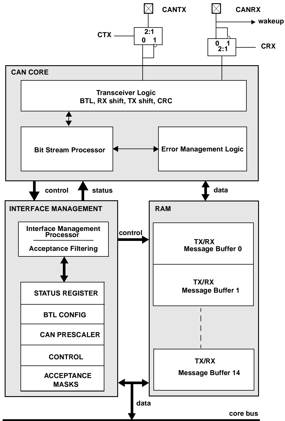
Figure 45. Block Diagram CR16CAN Interface
