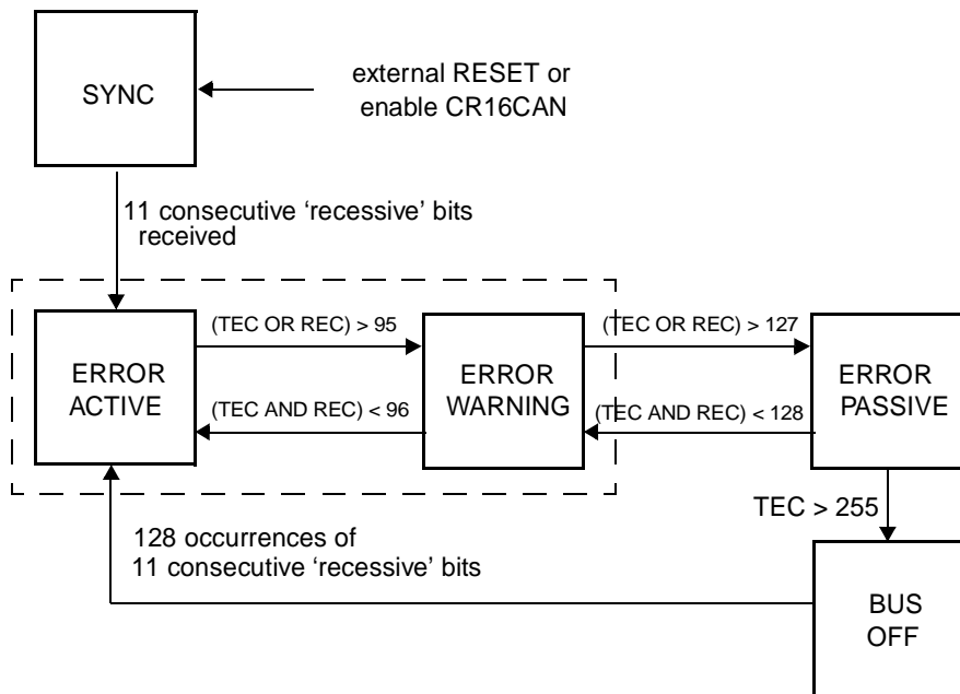
Figure 52. CR16CAN Bus States
