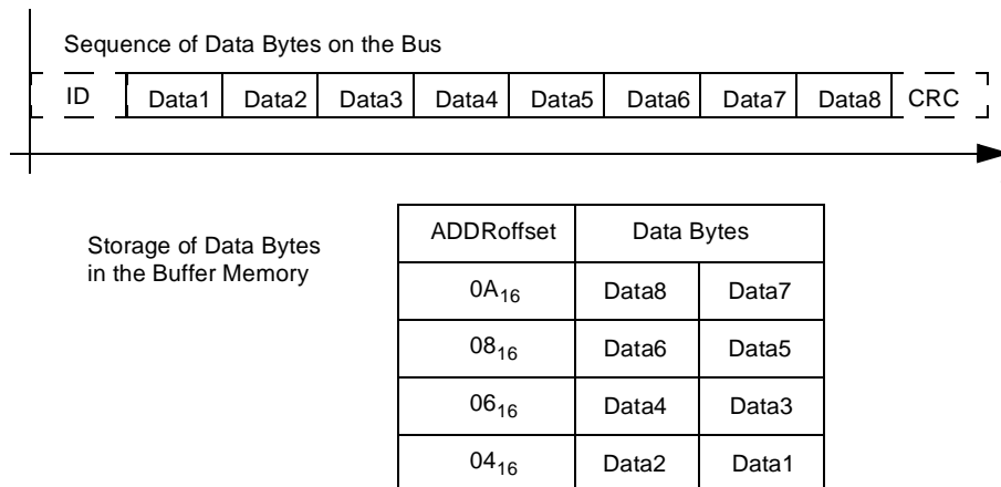
Figure 71. Data Direction Bit set to ‘1’
