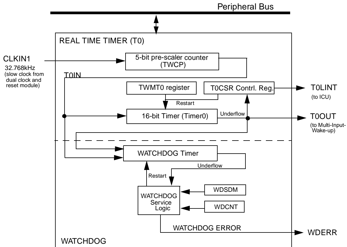
Figure 11. Timing and WATCHDOG Module Block Diagram
