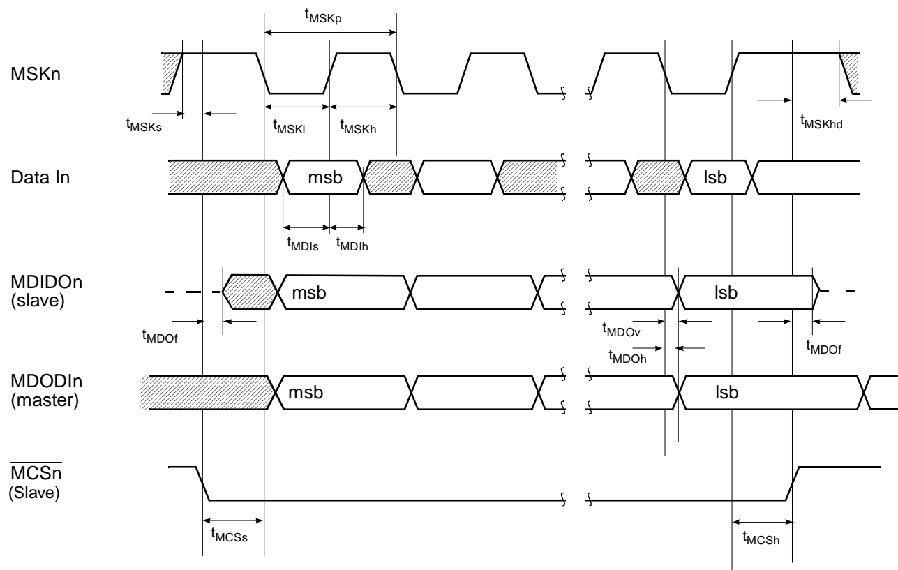
Figure 86. MICROWIRE Transaction Timing, Normal Mode, MIDL bit = 1
