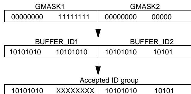
Figure 59. Acceptance of a Group of Identifiers
