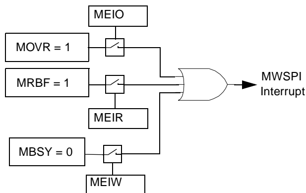
Figure 31. MWSPI Interrupts
