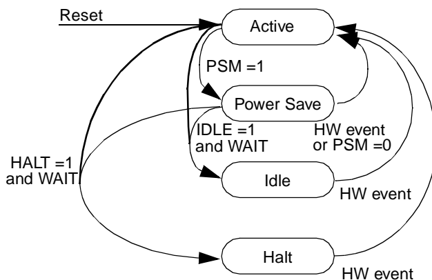
Figure 7. Power Modes and Transitions
