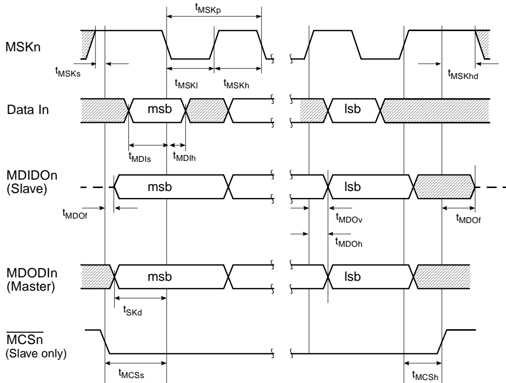
Figure 88. MICROWIRE Transaction Timing, Alternate Mode, MIDL bit = 1
