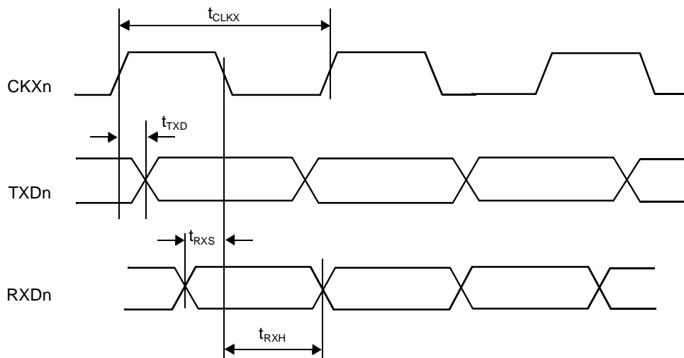
Figure 83. USART Synchronous Mode Timing
