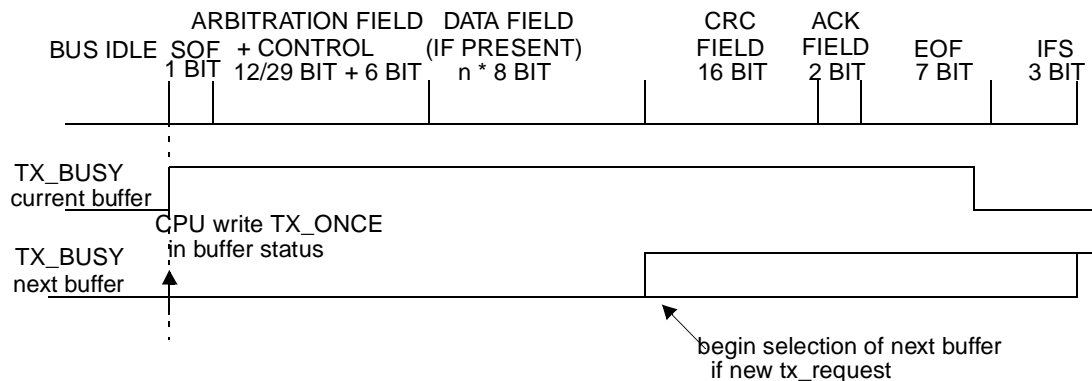
Figure 65. Data Transmission
