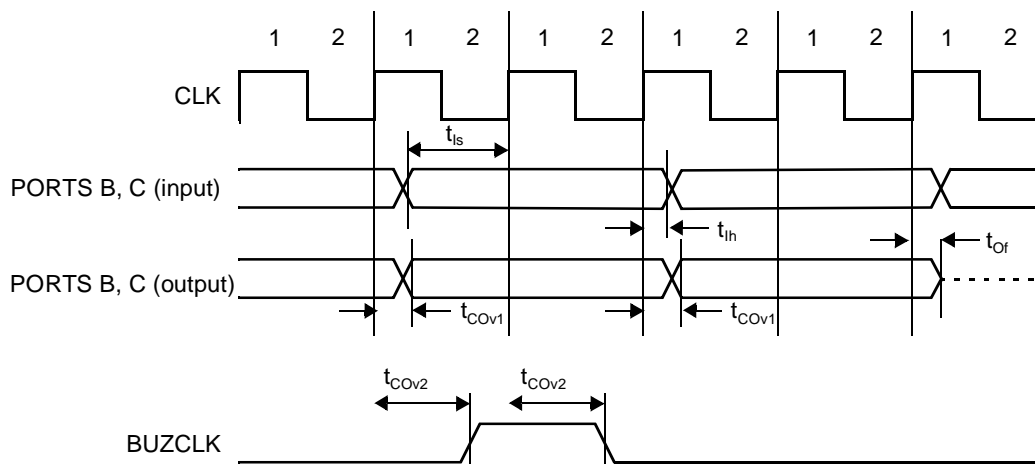
Figure 84. Ports Signals Timing
