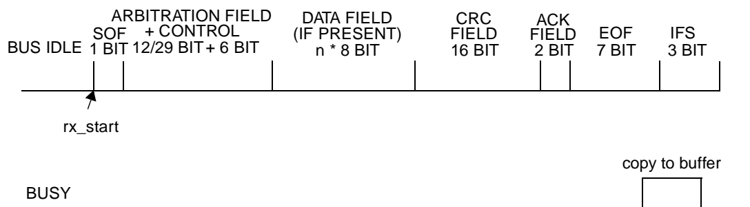
Figure 62. Receive Timing
