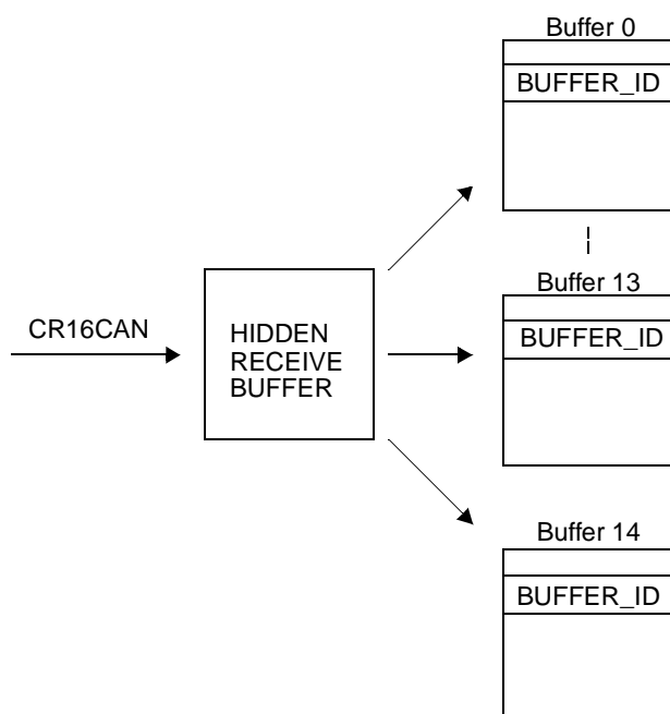
Figure 61. Receive Buffer Structure
