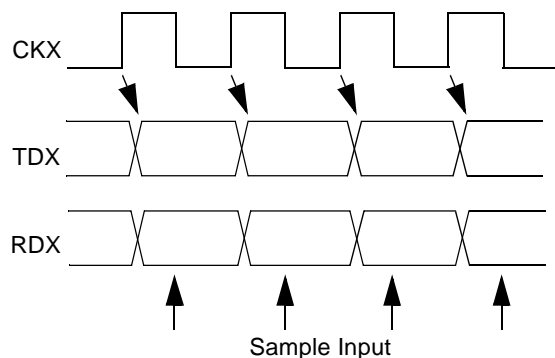
Figure 35. USART Synchronous Communication
