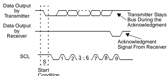
Figure 43. ACCESS.bus Acknowledge Cycle
