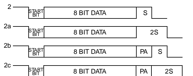
Figure 37. Eight Data Bit Frame Options
