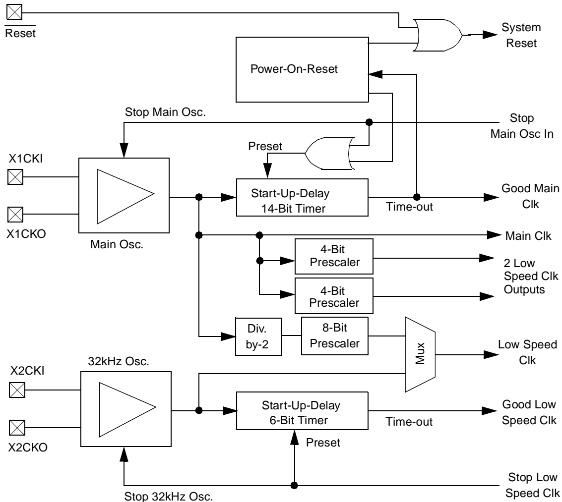
Figure 8. Dual Clock and Reset Module Block Diagram
