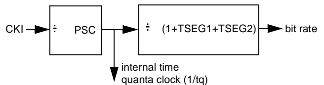
Figure 56. Bit Rate Generation
