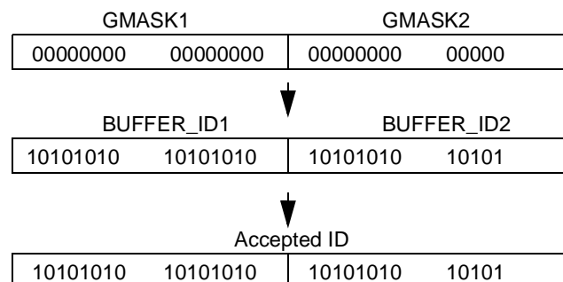
Figure 58. Acceptance of a Single Identifier
