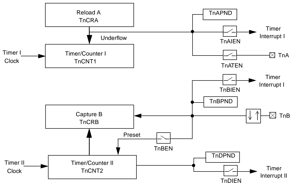
Figure 18. Mode 4: Input Capture Plus Timer Block Diagram
