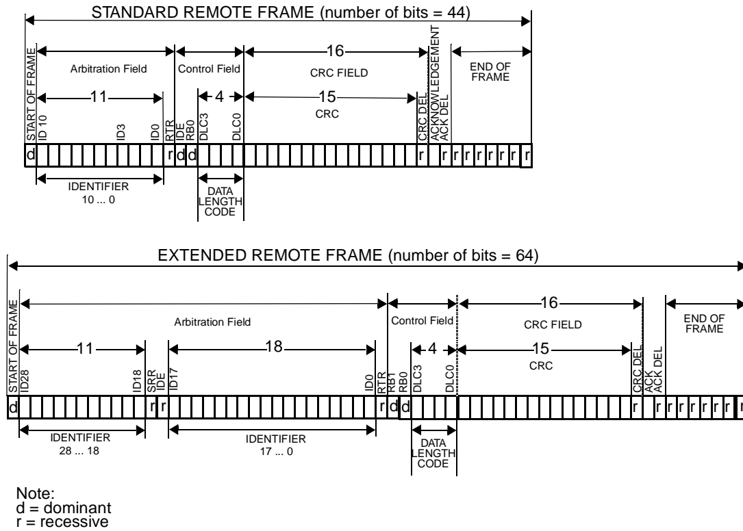
Figure 48. CAN Remote Frame (standard and extended)
