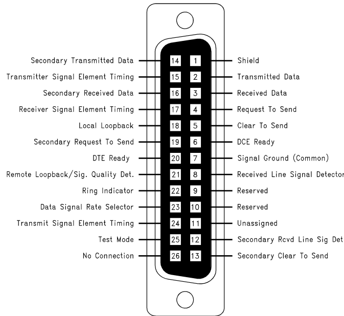
FIGURE 2. RS-232 ALT-A
