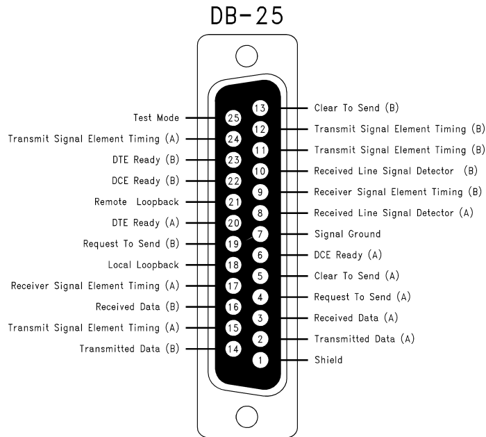
FIGURE 4. EIA-530 DB-25
