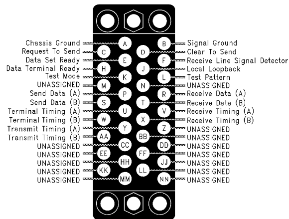
FIGURE 8. CCITT V.35
